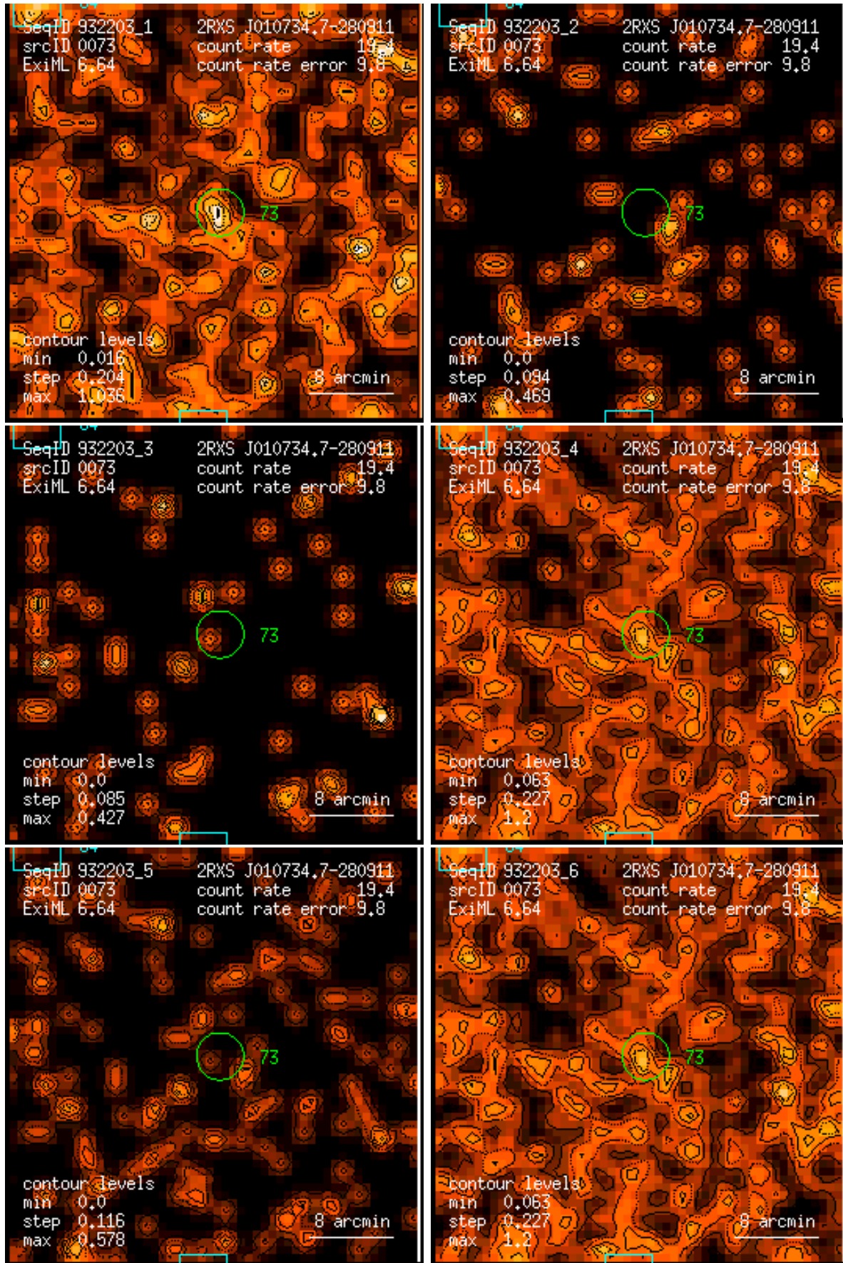
Figure 73: RASS 932203: detection 0073: band rate images, Gaussian filter: (1) PSPC channels 11 – 41, (2) 52 – 90, (3) 91 – 201, (4) 11 – 235, (5) 52 – 201, (6) 11 – 201. Broad band rates in counts/ks. Band rate contour levels in counts/ks/arcmin 2 .
