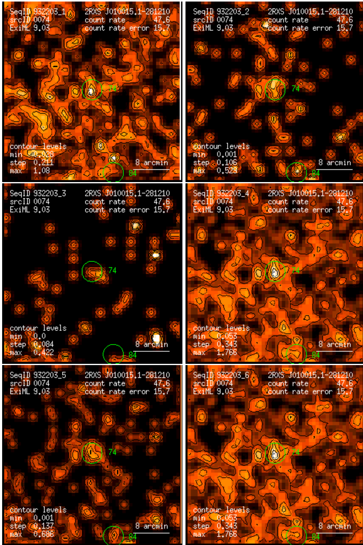
Figure 74: RASS 932203: detection 0074: band rate images, Gaussian filter: (1) PSPC channels 11 – 41, (2) 52 – 90, (3) 91 – 201, (4) 11 – 235, (5) 52 – 201, (6) 11 – 201. Broad band rates in counts/ks. Band rate contour levels in counts/ks/arcmin 2 .
