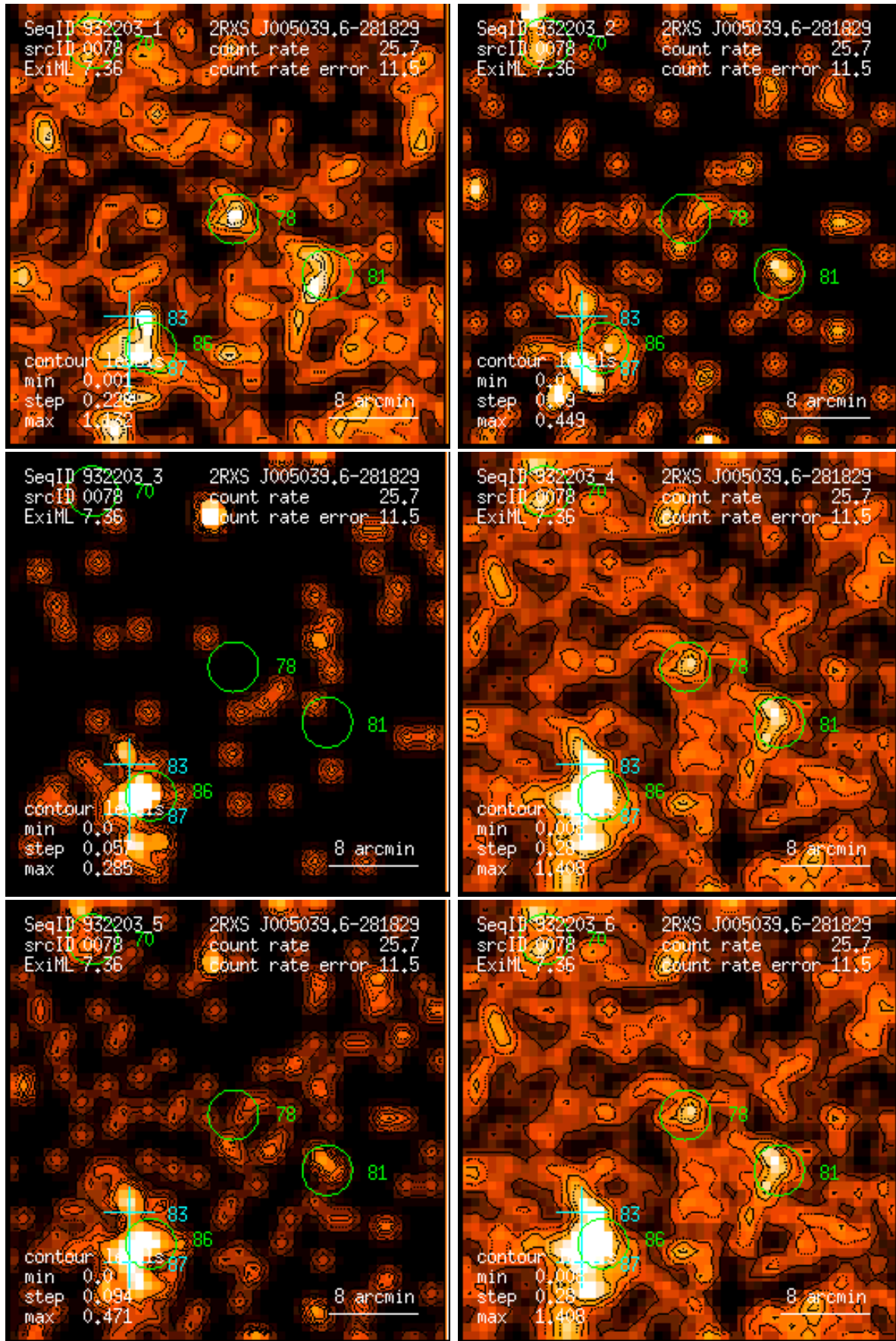
Figure 78: RASS 932203: detection 0078: band rate images, Gaussian filter: (1) PSPC channels 11 – 41, (2) 52 – 90, (3) 91 – 201, (4) 11 – 235, (5) 52 – 201, (6) 11 – 201. Broad band rates in counts/ks. Band rate contour levels in counts/ks/arcmin 2 .
