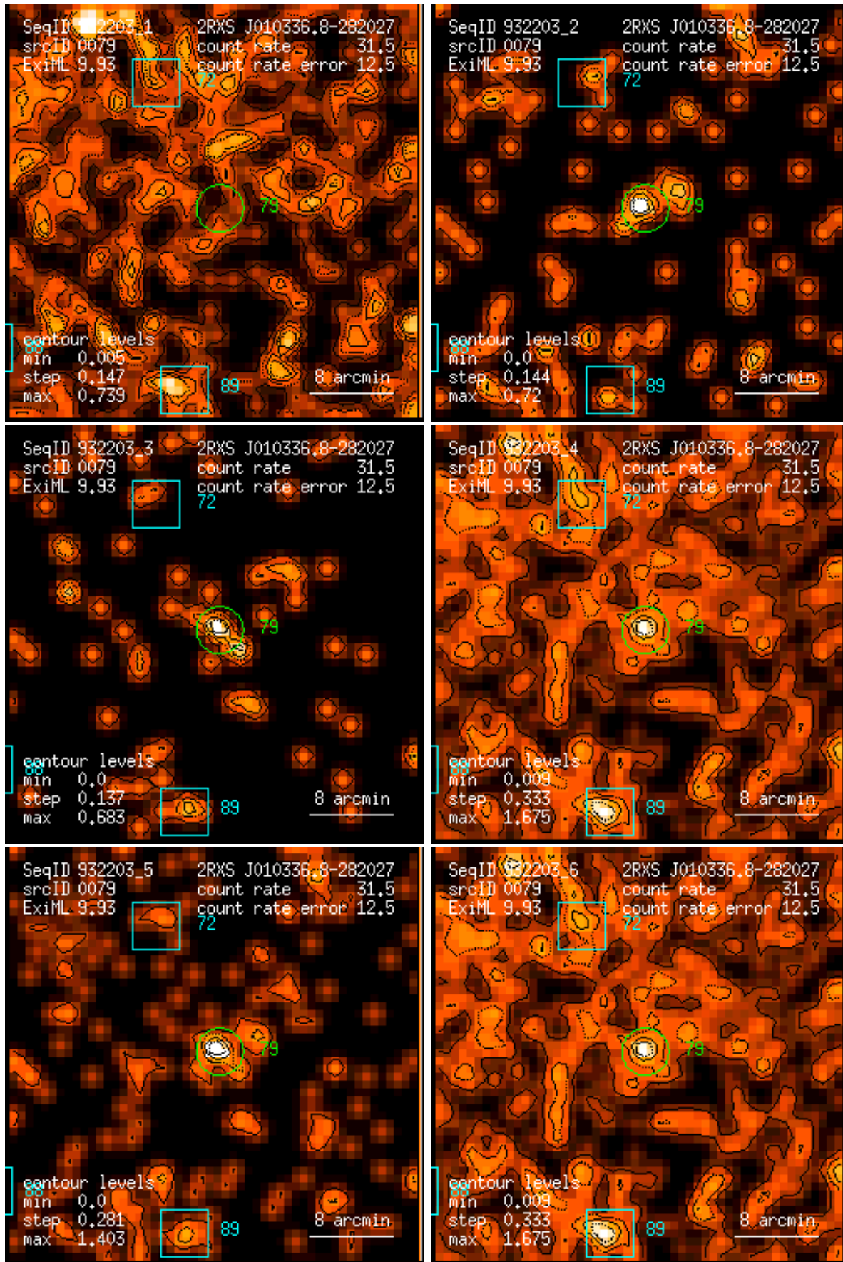
Figure 79: RASS 932203: detection 0079: band rate images, Gaussian filter: (1) PSPC channels 11 – 41, (2) 52 – 90, (3) 91 – 201, (4) 11 – 235, (5) 52 – 201, (6) 11 – 201. Broad band rates in counts/ks. Band rate contour levels in counts/ks/arcmin 2 .
