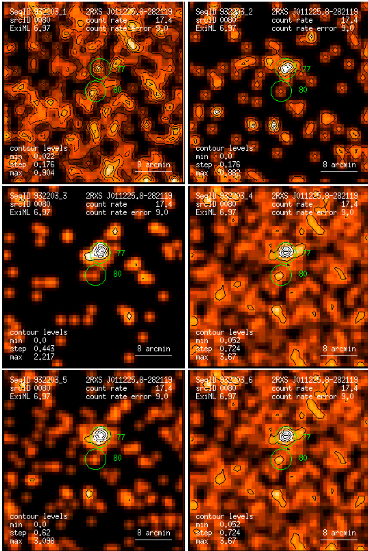
Figure 80: RASS 932203: detection 0080: band rate images, Gaussian filter: (1) PSPC channels 11 – 41, (2) 52 – 90, (3) 91 – 201, (4) 11 – 235, (5) 52 – 201, (6) 11 – 201. Broad band rates in counts/ks. Band rate contour levels in counts/ks/arcmin 2 .
