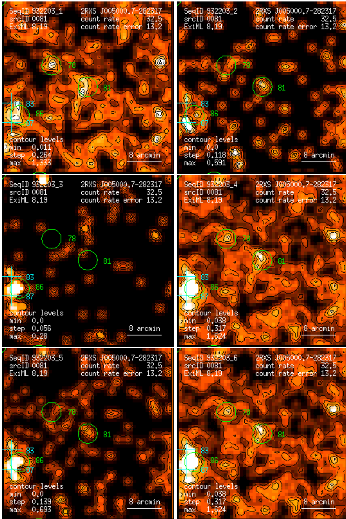
Figure 81: RASS 932203: detection 0081: band rate images, Gaussian filter: (1) PSPC channels 11 – 41, (2) 52 – 90, (3) 91 – 201, (4) 11 – 235, (5) 52 – 201, (6) 11 – 201. Broad band rates in counts/ks. Band rate contour levels in counts/ks/arcmin 2 .
