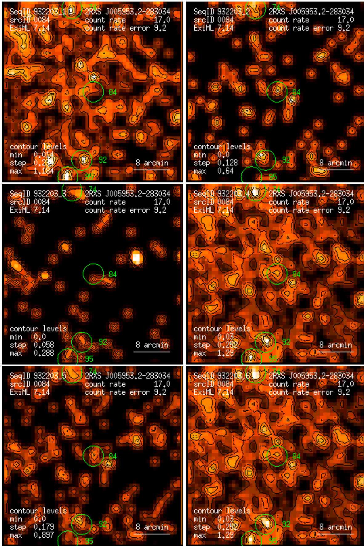
Figure 84: RASS 932203: detection 0084: band rate images, Gaussian filter: (1) PSPC channels 11 – 41, (2) 52 – 90, (3) 91 – 201, (4) 11 – 235, (5) 52 – 201, (6) 11 – 201. Broad band rates in counts/ks. Band rate contour levels in counts/ks/arcmin 2 .
