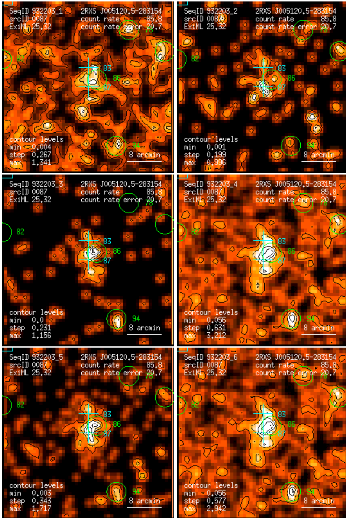
Figure 87: RASS 932203: detection 0087: band rate images, Gaussian filter: (1) PSPC channels 11 – 41, (2) 52 – 90, (3) 91 – 201, (4) 11 – 235, (5) 52 – 201, (6) 11 – 201. Broad band rates in counts/ks. Band rate contour levels in counts/ks/arcmin 2 .
