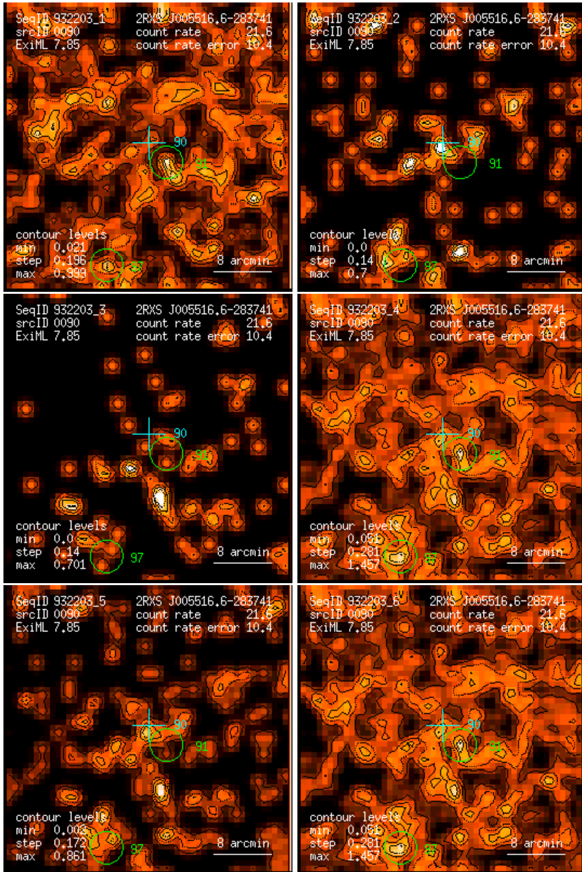
Figure 90: RASS 932203: detection 0090: band rate images, Gaussian filter: (1) PSPC channels 11 – 41, (2) 52 – 90, (3) 91 – 201, (4) 11 – 235, (5) 52 – 201, (6) 11 – 201. Broad band rates in counts/ks. Band rate contour levels in counts/ks/arcmin 2 .
