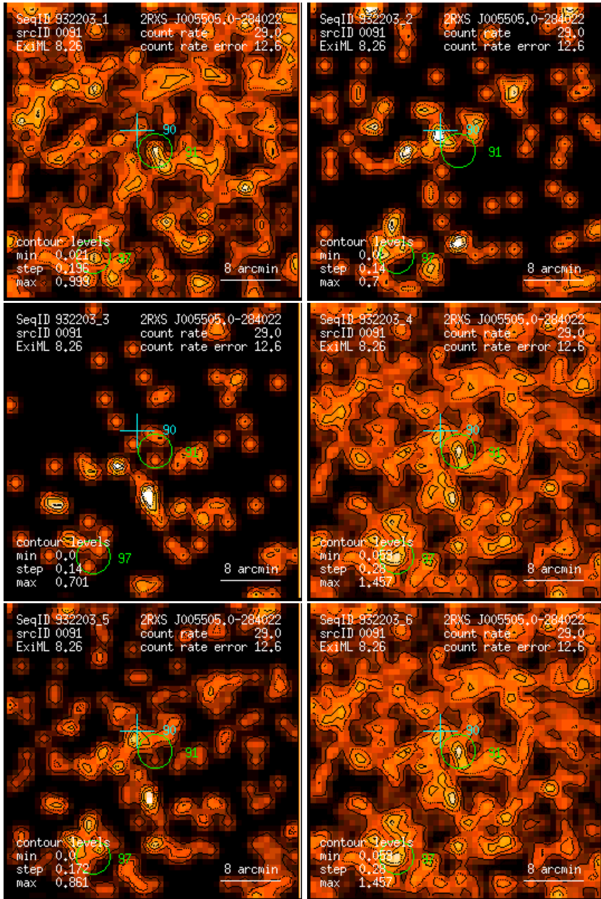
Figure 91: RASS 932203: detection 0091: band rate images, Gaussian filter: (1) PSPC channels 11 – 41, (2) 52 – 90, (3) 91 – 201, (4) 11 – 235, (5) 52 – 201, (6) 11 – 201. Broad band rates in counts/ks. Band rate contour levels in counts/ks/arcmin 2 .
