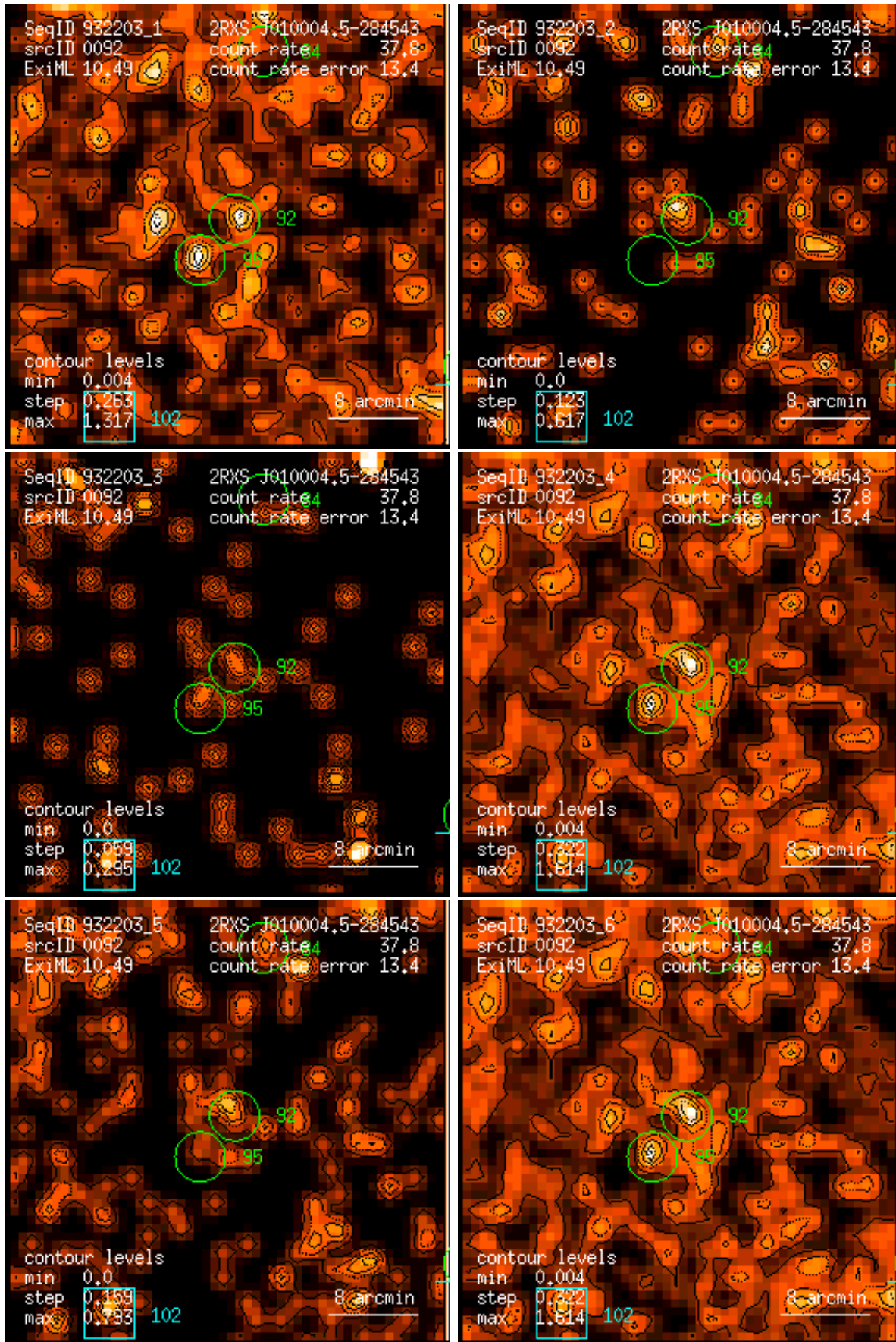
Figure 92: RASS 932203: detection 0092: band rate images, Gaussian filter: (1) PSPC channels 11 – 41, (2) 52 – 90, (3) 91 – 201, (4) 11 – 235, (5) 52 – 201, (6) 11 – 201. Broad band rates in counts/ks. Band rate contour levels in counts/ks/arcmin 2 .
