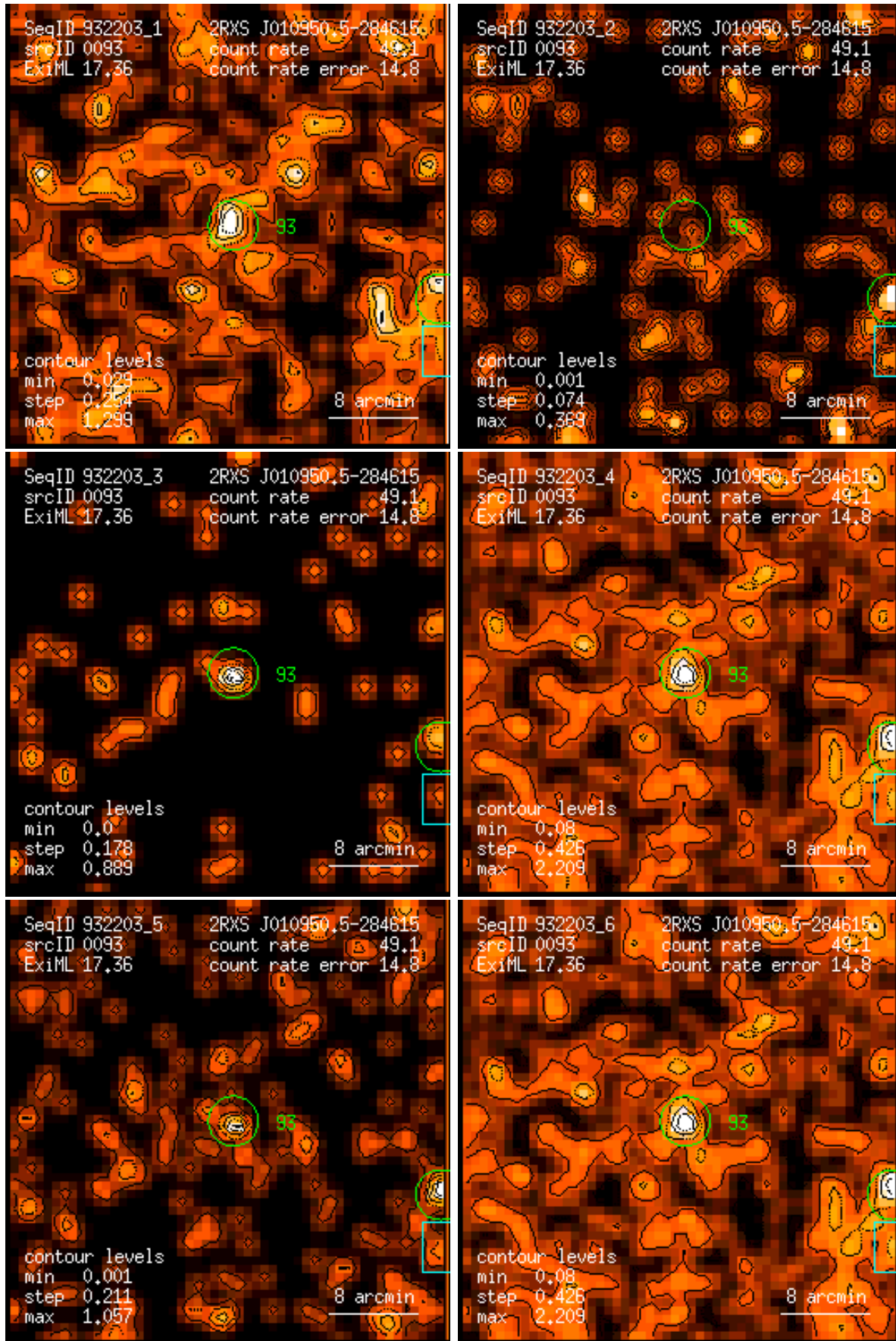
Figure 93: RASS 932203: detection 0093: band rate images, Gaussian filter: (1) PSPC channels 11 – 41, (2) 52 – 90, (3) 91 – 201, (4) 11 – 235, (5) 52 – 201, (6) 11 – 201. Broad band rates in counts/ks. Band rate contour levels in counts/ks/arcmin 2 .
