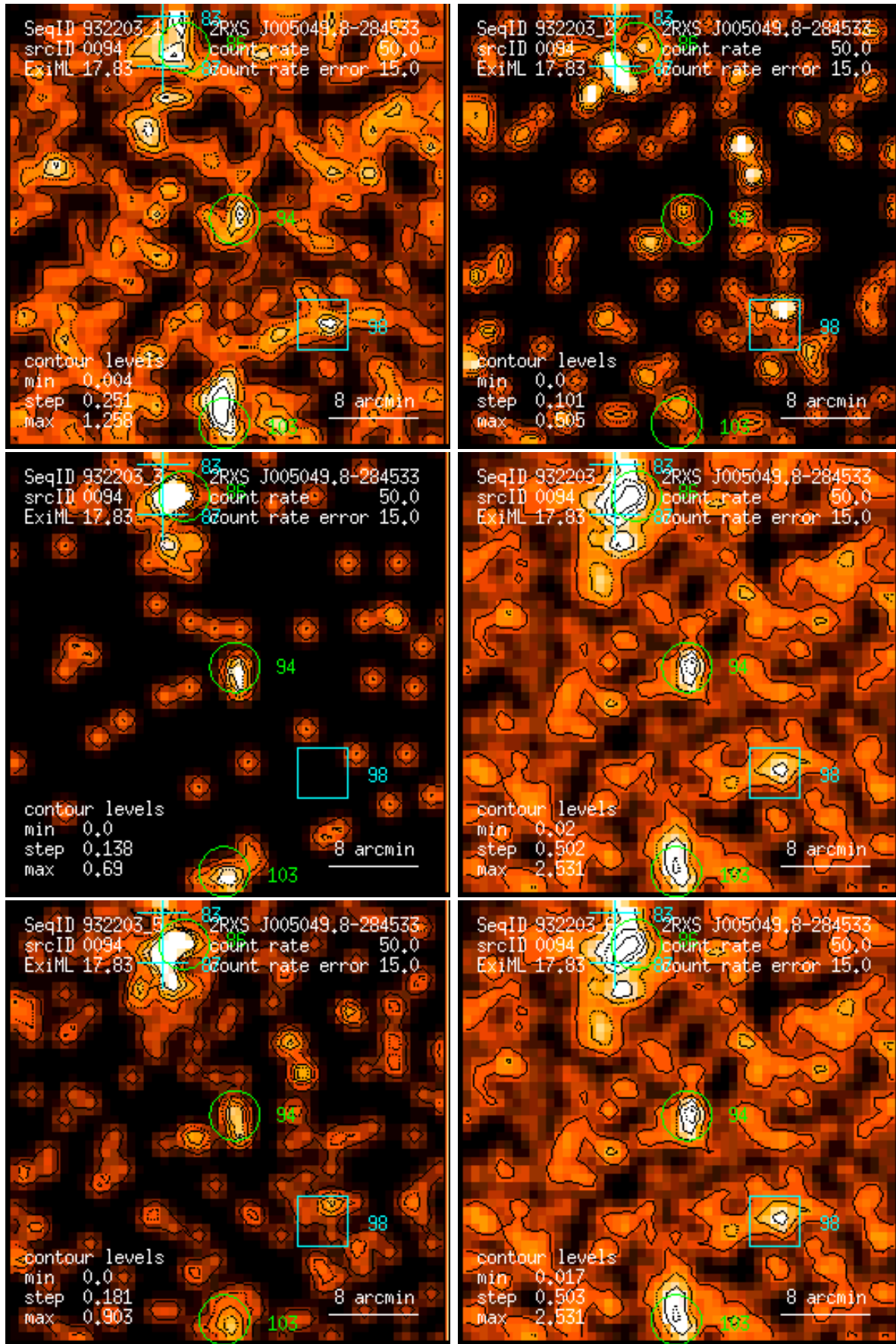
Figure 94: RASS 932203: detection 0094: band rate images, Gaussian filter: (1) PSPC channels 11 – 41, (2) 52 – 90, (3) 91 – 201, (4) 11 – 235, (5) 52 – 201, (6) 11 – 201. Broad band rates in counts/ks. Band rate contour levels in counts/ks/arcmin 2 .
