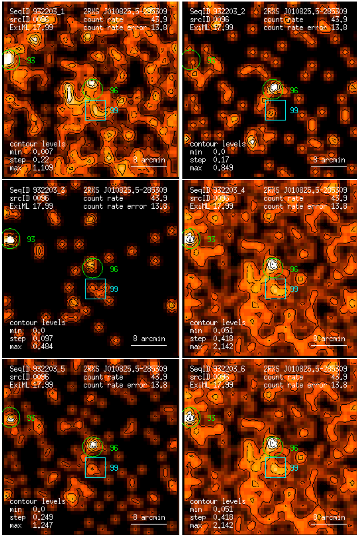
Figure 96: RASS 932203: detection 0096: band rate images, Gaussian filter: (1) PSPC channels 11 – 41, (2) 52 – 90, (3) 91 – 201, (4) 11 – 235, (5) 52 – 201, (6) 11 – 201. Broad band rates in counts/ks. Band rate contour levels in counts/ks/arcmin 2 .
