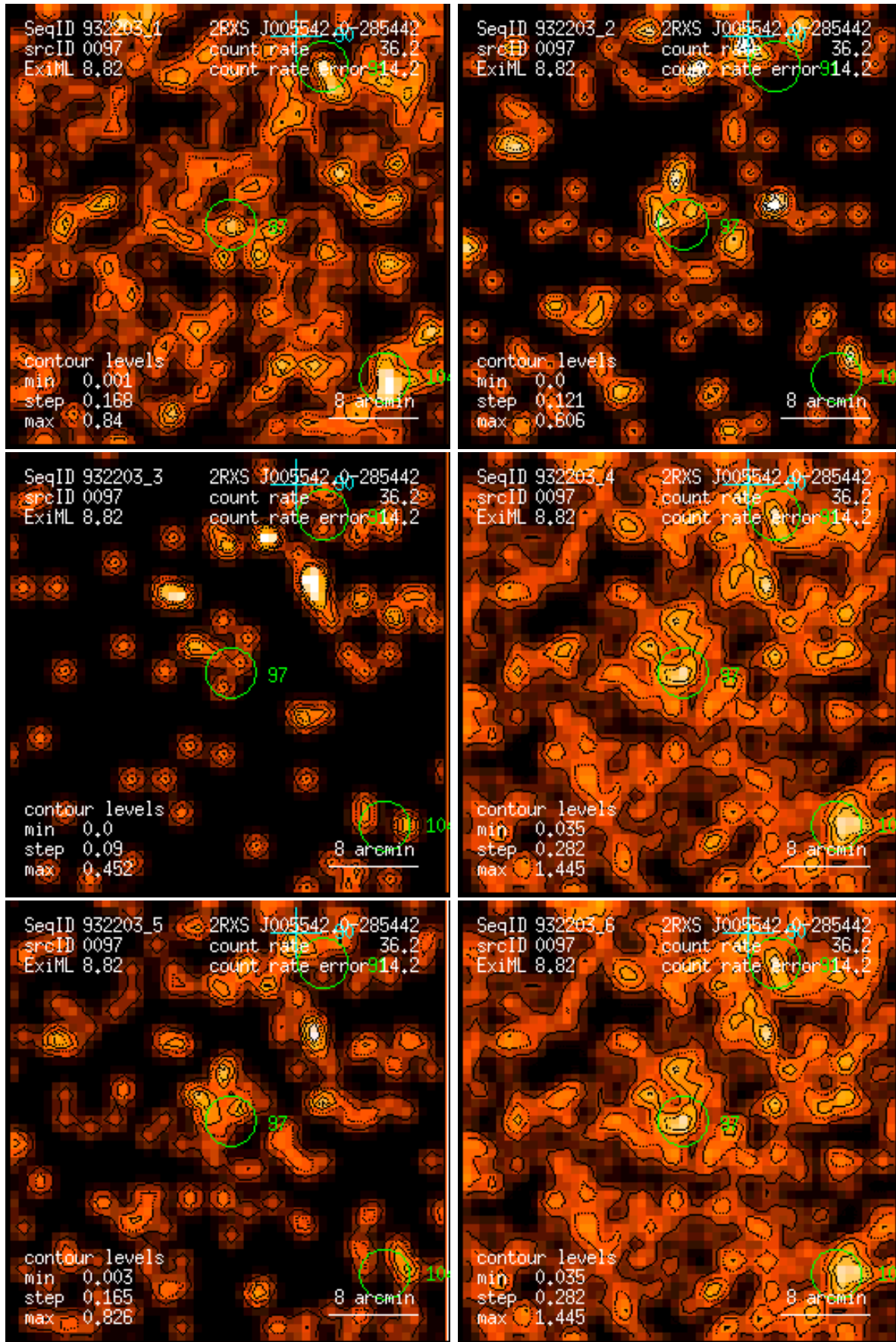
Figure 97: RASS 932203: detection 0097: band rate images, Gaussian filter: (1) PSPC channels 11 – 41, (2) 52 – 90, (3) 91 – 201, (4) 11 – 235, (5) 52 – 201, (6) 11 – 201. Broad band rates in counts/ks. Band rate contour levels in counts/ks/arcmin 2 .
