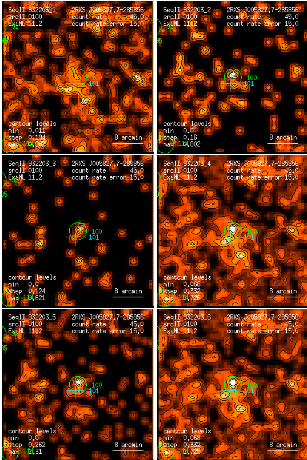
Figure 100: RASS 932203: detection 0100: band rate images, Gaussian filter: (1) PSPC channels 11 – 41, (2) 52 – 90, (3) 91 – 201, (4) 11 – 235, (5) 52 – 201, (6) 11 – 201. Broad band rates in counts/ks. Band rate contour levels in counts/ks/arcmin 2 .
