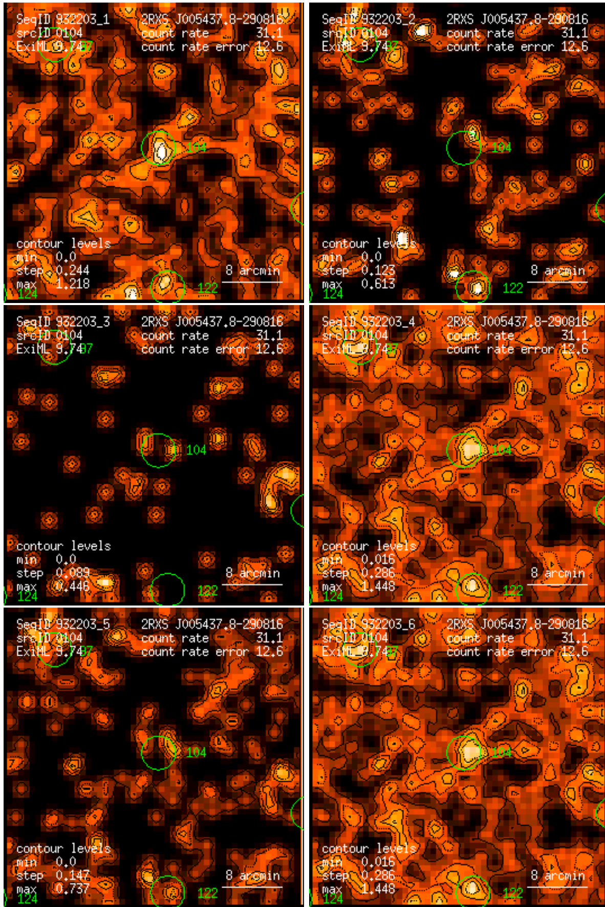
Figure 104: RASS 932203: detection 0104: band rate images, Gaussian filter: (1) PSPC channels 11 – 41, (2) 52 – 90, (3) 91 – 201, (4) 11 – 235, (5) 52 – 201, (6) 11 – 201. Broad band rates in counts/ks. Band rate contour levels in counts/ks/arcmin 2 .
