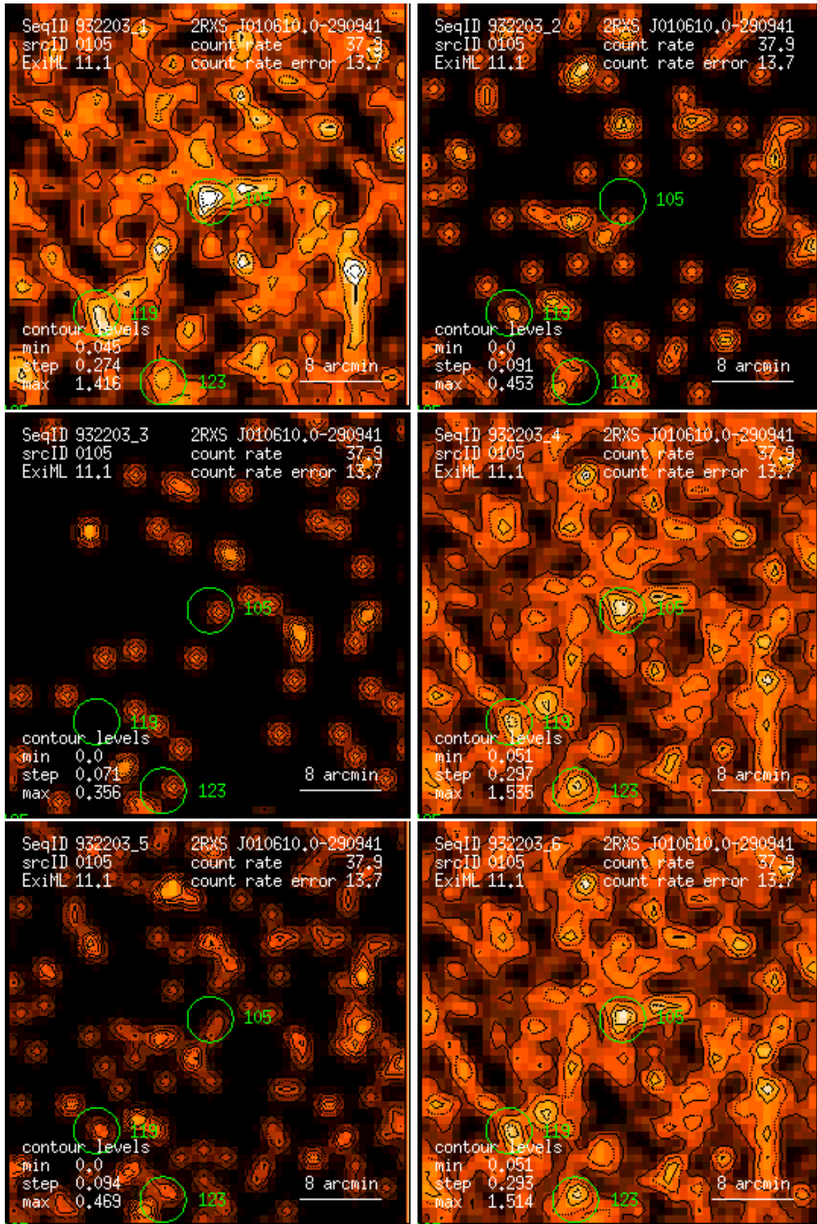
Figure 105: RASS 932203: detection 0105: band rate images, Gaussian filter: (1) PSPC channels 11 – 41, (2) 52 – 90, (3) 91 – 201, (4) 11 – 235, (5) 52 – 201, (6) 11 – 201. Broad band rates in counts/ks. Band rate contour levels in counts/ks/arcmin 2 .
