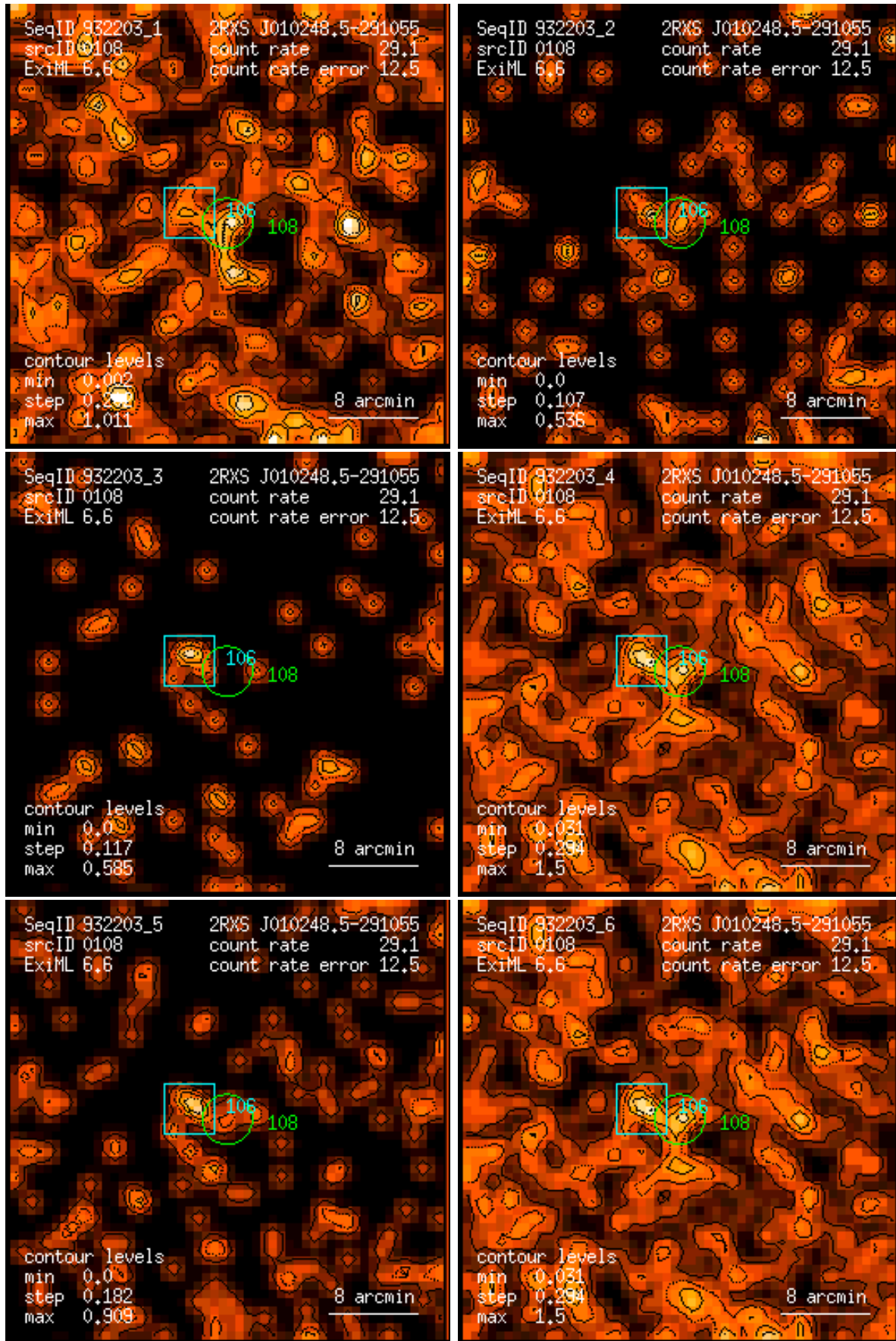
Figure 108: RASS 932203: detection 0108: band rate images, Gaussian filter: (1) PSPC channels 11 – 41, (2) 52 – 90, (3) 91 – 201, (4) 11 – 235, (5) 52 – 201, (6) 11 – 201. Broad band rates in counts/ks. Band rate contour levels in counts/ks/arcmin 2 .
