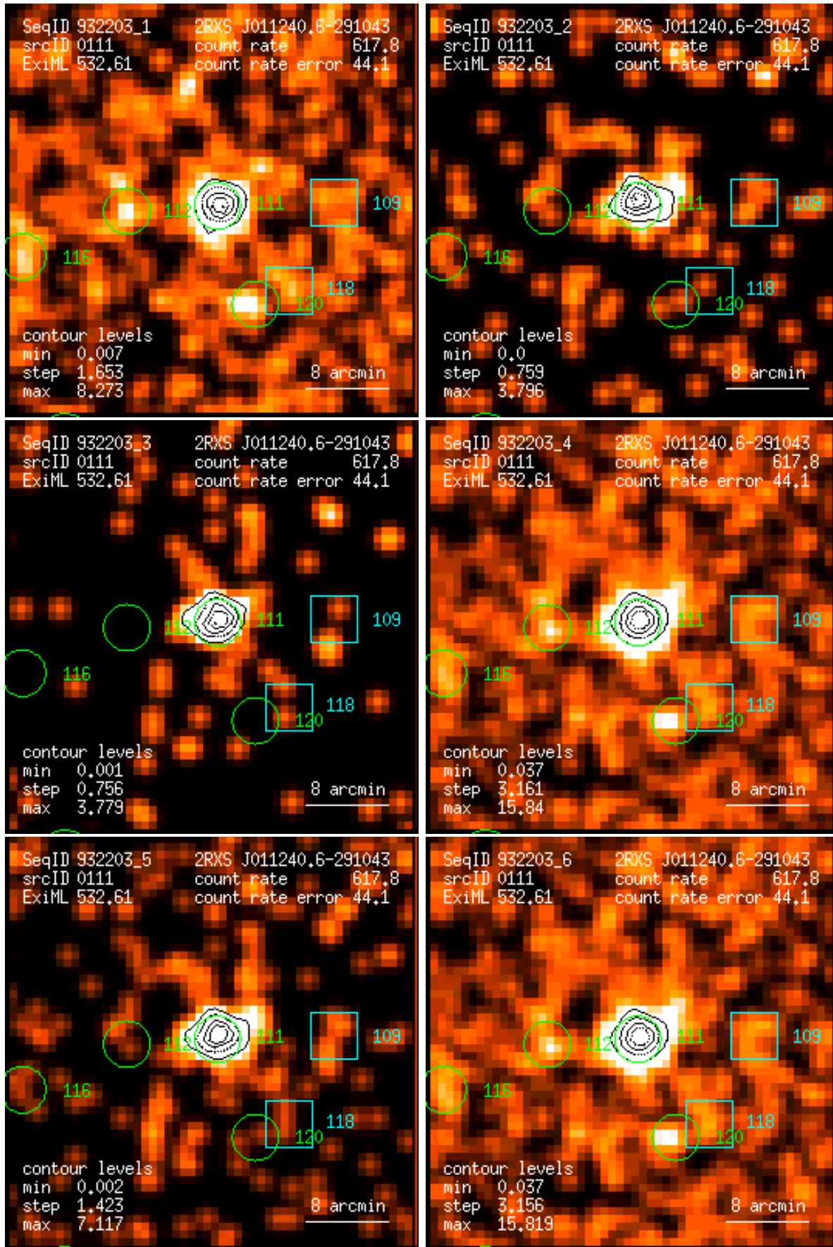
Figure 111: RASS 932203: detection 0111: band rate images, Gaussian filter: (1) PSPC channels 11 – 41, (2) 52 – 90, (3) 91 – 201, (4) 11 – 235, (5) 52 – 201, (6) 11 – 201. Broad band rates in counts/ks. Band rate contour levels in counts/ks/arcmin 2 .
