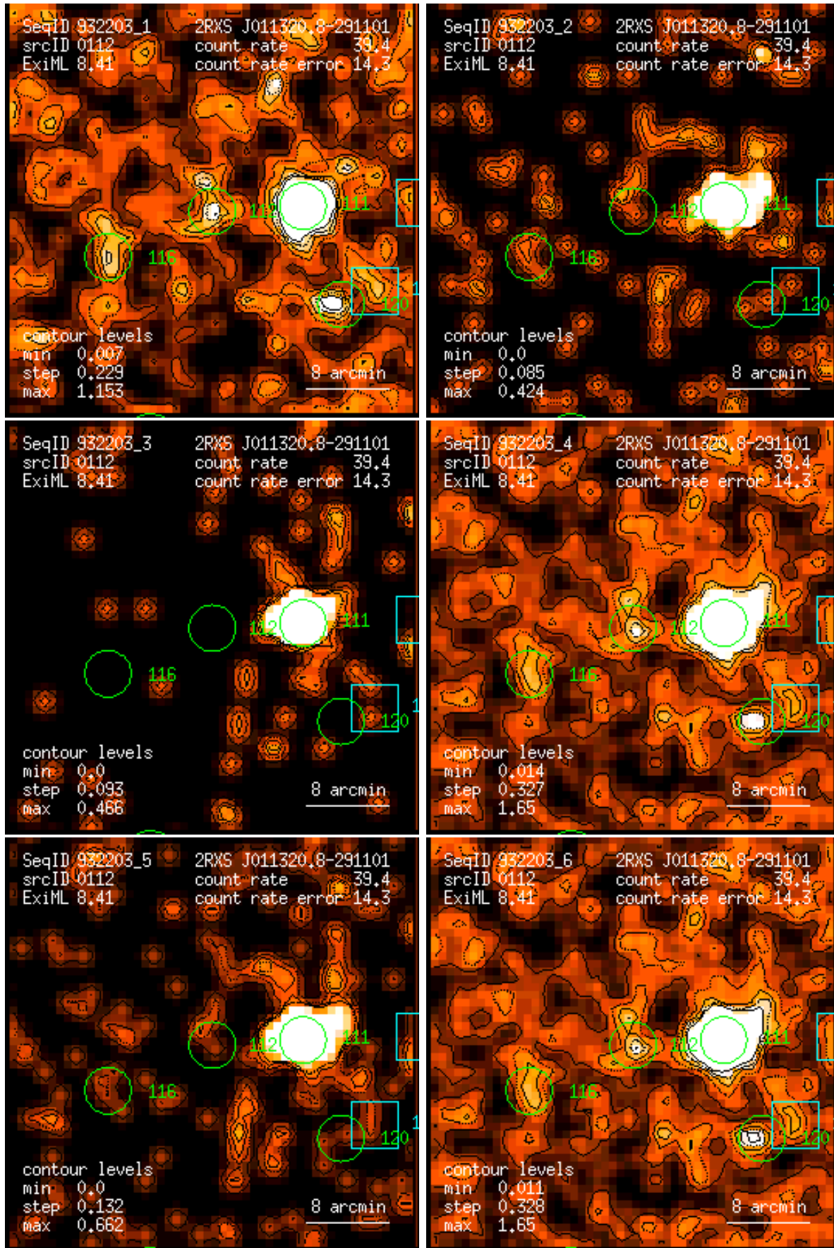
Figure 112: RASS 932203: detection 0112: band rate images, Gaussian filter: (1) PSPC channels 11 – 41, (2) 52 – 90, (3) 91 – 201, (4) 11 – 235, (5) 52 – 201, (6) 11 – 201. Broad band rates in counts/ks. Band rate contour levels in counts/ks/arcmin 2 .
