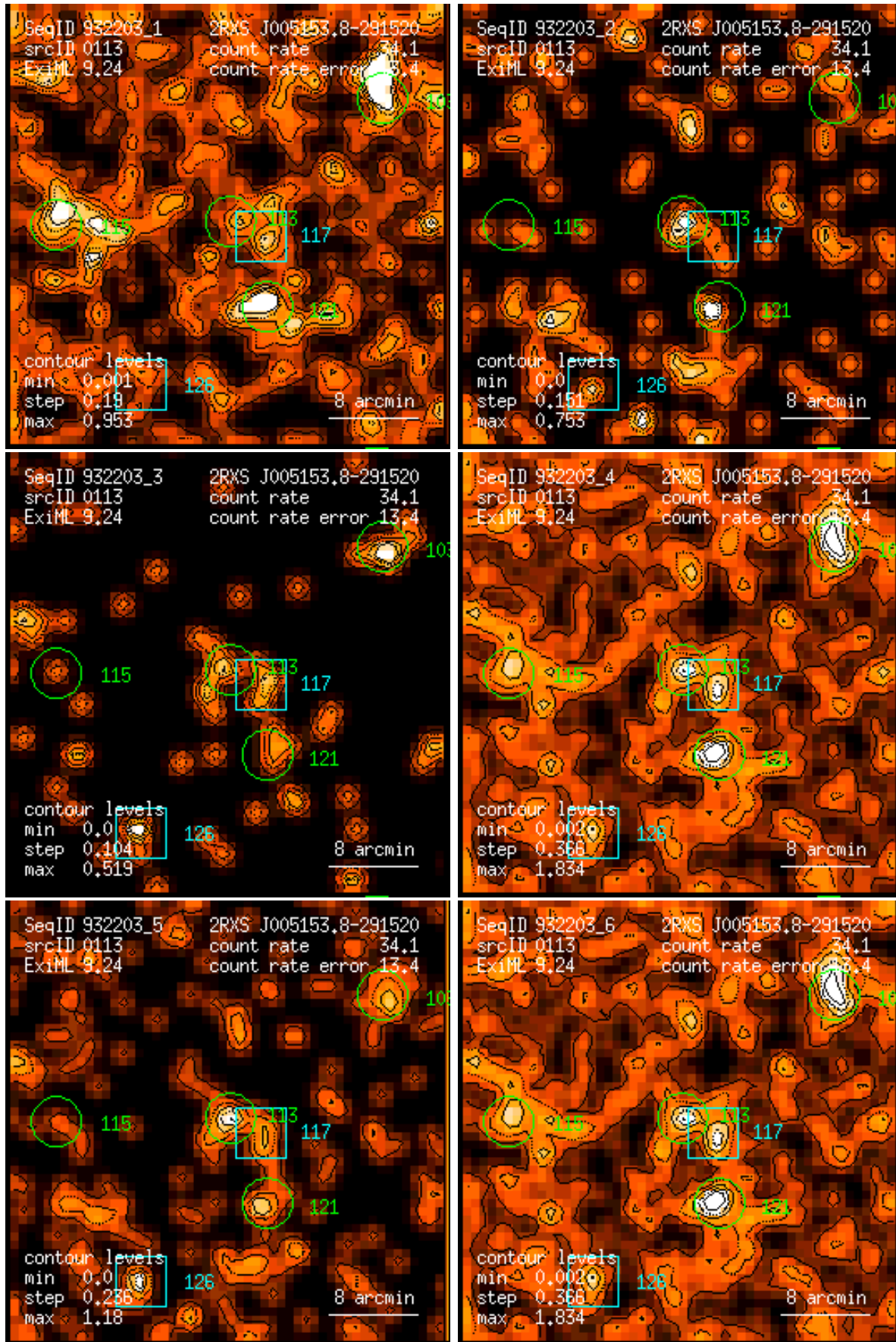
Figure 113: RASS 932203: detection 0113: band rate images, Gaussian filter: (1) PSPC channels 11 – 41, (2) 52 – 90, (3) 91 – 201, (4) 11 – 235, (5) 52 – 201, (6) 11 – 201. Broad band rates in counts/ks. Band rate contour levels in counts/ks/arcmin 2 .
