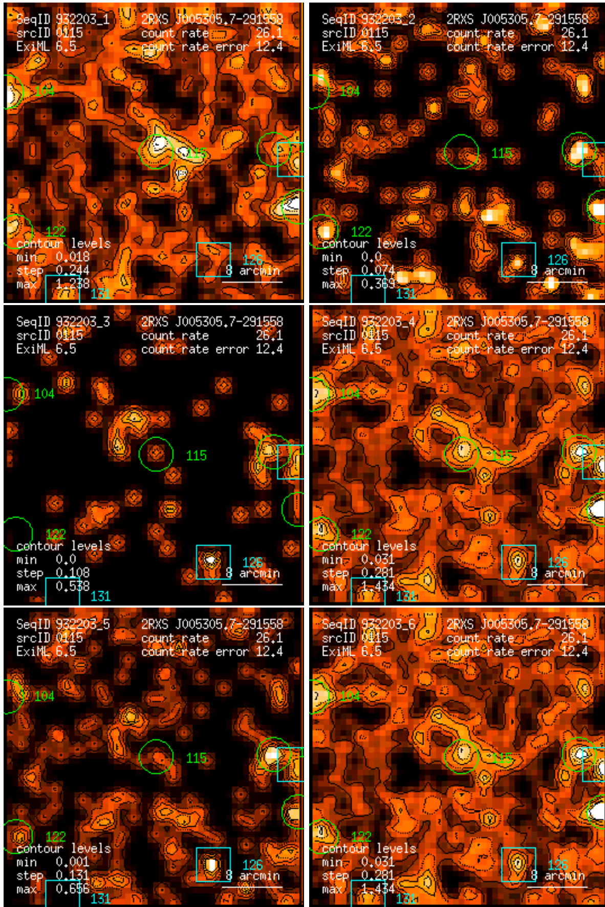
Figure 115: RASS 932203: detection 0115: band rate images, Gaussian filter: (1) PSPC channels 11 – 41, (2) 52 – 90, (3) 91 – 201, (4) 11 – 235, (5) 52 – 201, (6) 11 – 201. Broad band rates in counts/ks. Band rate contour levels in counts/ks/arcmin 2 .
