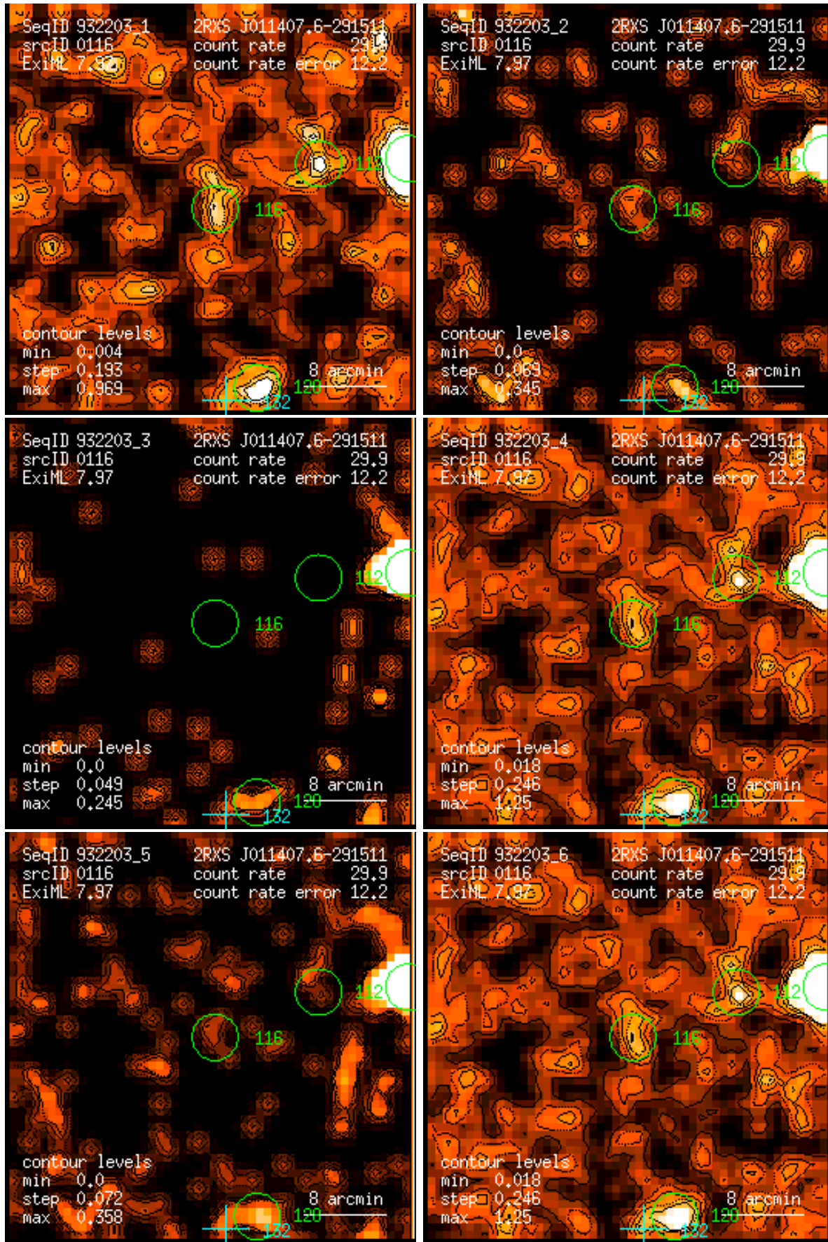
Figure 116: RASS 932203: detection 0116: band rate images, Gaussian filter: (1) PSPC channels 11 – 41, (2) 52 – 90, (3) 91 – 201, (4) 11 – 235, (5) 52 – 201, (6) 11 – 201. Broad band rates in counts/ks. Band rate contour levels in counts/ks/arcmin 2 .
