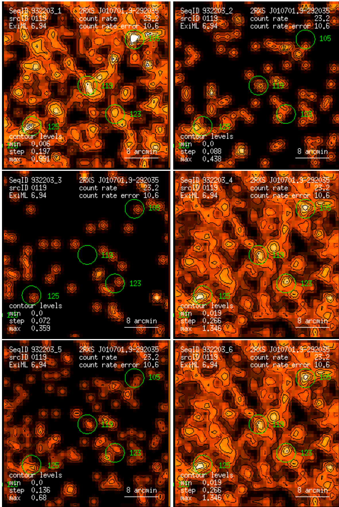
Figure 119: RASS 932203: detection 0119: band rate images, Gaussian filter: (1) PSPC channels 11 – 41, (2) 52 – 90, (3) 91 – 201, (4) 11 – 235, (5) 52 – 201, (6) 11 – 201. Broad band rates in counts/ks. Band rate contour levels in counts/ks/arcmin 2 .
