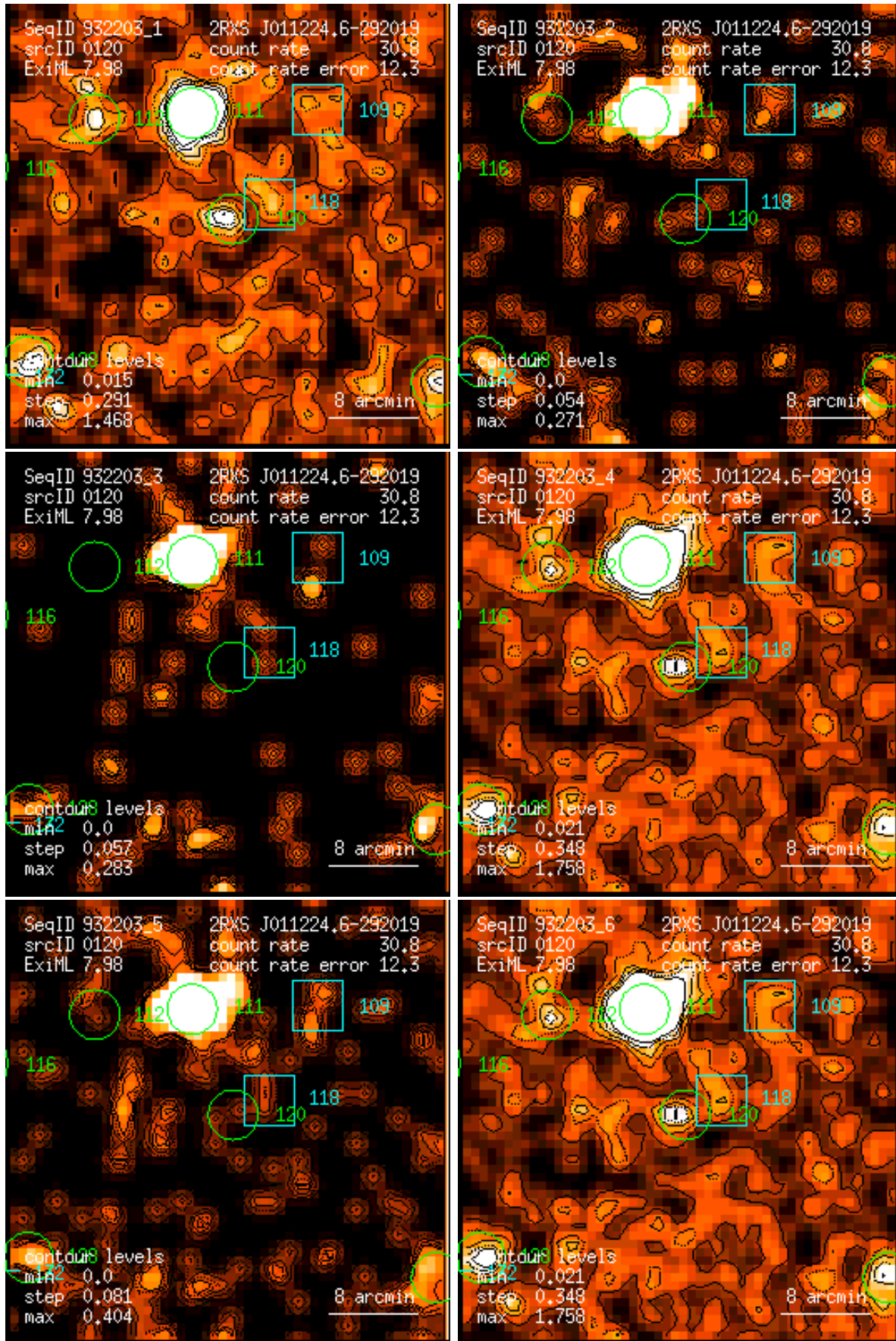
Figure 120: RASS 932203: detection 0120: band rate images, Gaussian filter: (1) PSPC channels 11 – 41, (2) 52 – 90, (3) 91 – 201, (4) 11 – 235, (5) 52 – 201, (6) 11 – 201. Broad band rates in counts/ks. Band rate contour levels in counts/ks/arcmin 2 .
