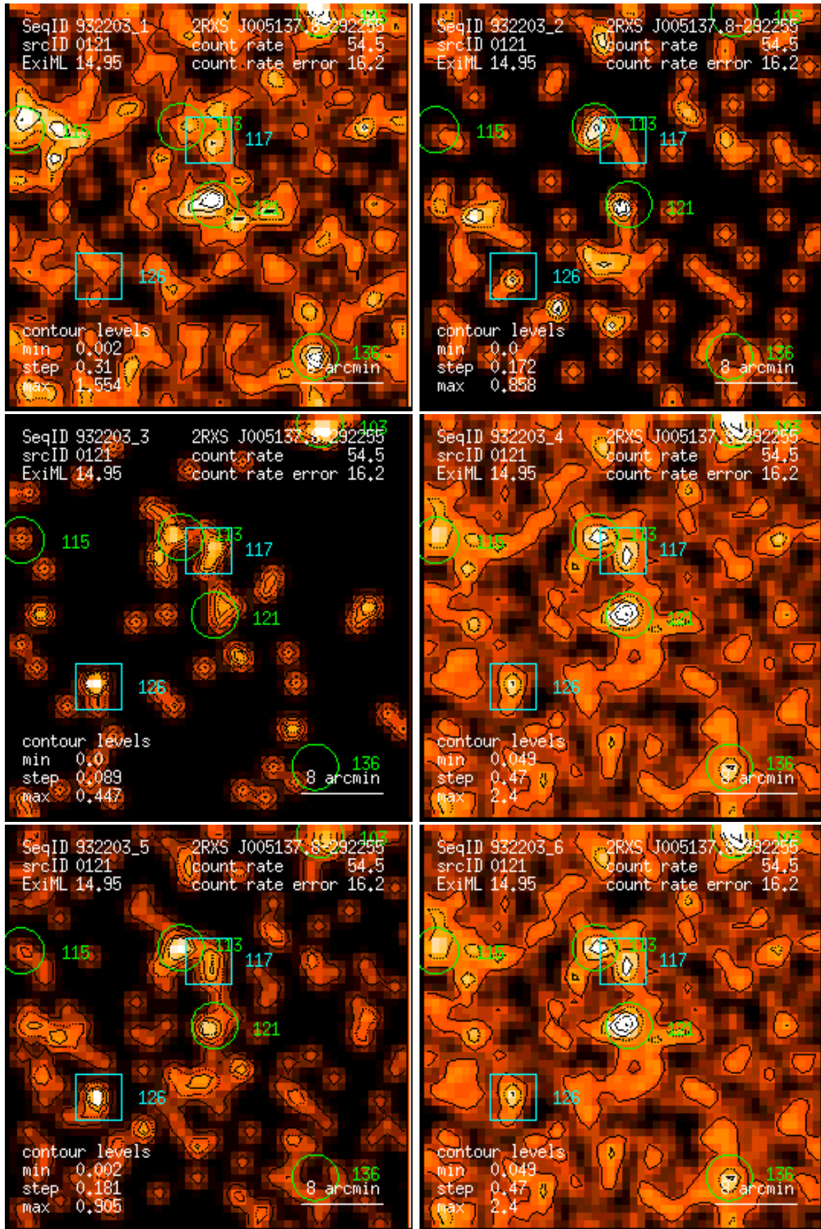
Figure 121: RASS 932203: detection 0121: band rate images, Gaussian filter: (1) PSPC channels 11 – 41, (2) 52 – 90, (3) 91 – 201, (4) 11 – 235, (5) 52 – 201, (6) 11 – 201. Broad band rates in counts/ks. Band rate contour levels in counts/ks/arcmin 2 .
