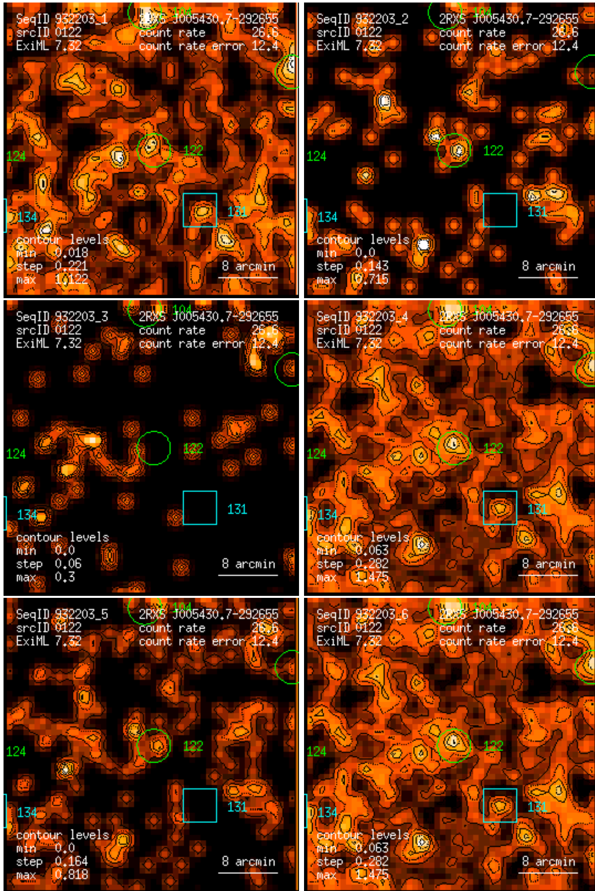
Figure 122: RASS 932203: detection 0122: band rate images, Gaussian filter: (1) PSPC channels 11 – 41, (2) 52 – 90, (3) 91 – 201, (4) 11 – 235, (5) 52 – 201, (6) 11 – 201. Broad band rates in counts/ks. Band rate contour levels in counts/ks/arcmin 2 .
