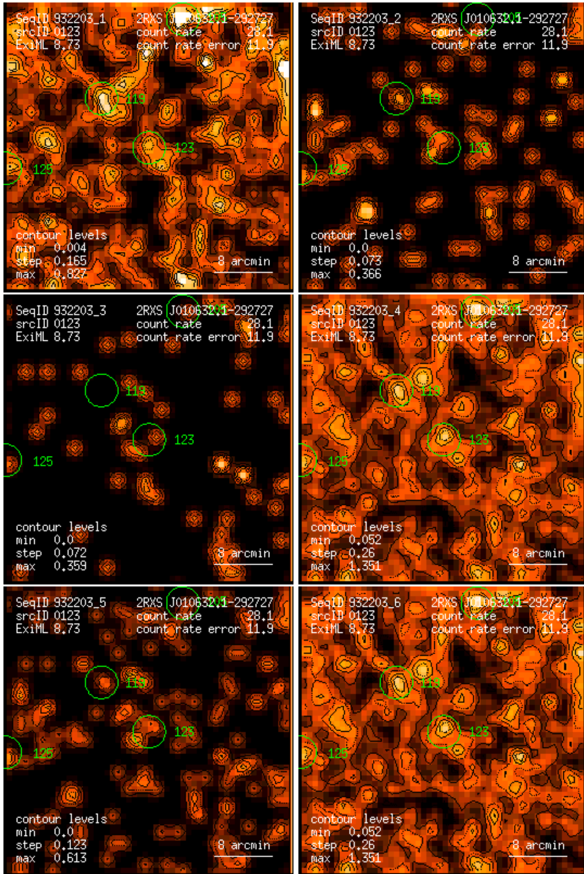
Figure 123: RASS 932203: detection 0123: band rate images, Gaussian filter: (1) PSPC channels 11 – 41, (2) 52 – 90, (3) 91 – 201, (4) 11 – 235, (5) 52 – 201, (6) 11 – 201. Broad band rates in counts/ks. Band rate contour levels in counts/ks/arcmin 2 .
