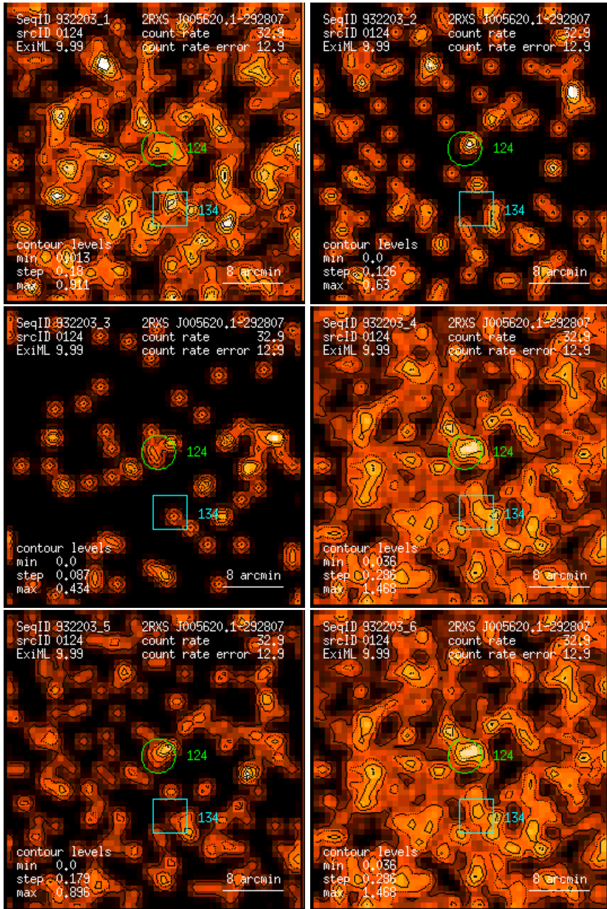
Figure 124: RASS 932203: detection 0124: band rate images, Gaussian filter: (1) PSPC channels 11 – 41, (2) 52 – 90, (3) 91 – 201, (4) 11 – 235, (5) 52 – 201, (6) 11 – 201. Broad band rates in counts/ks. Band rate contour levels in counts/ks/arcmin 2 .
