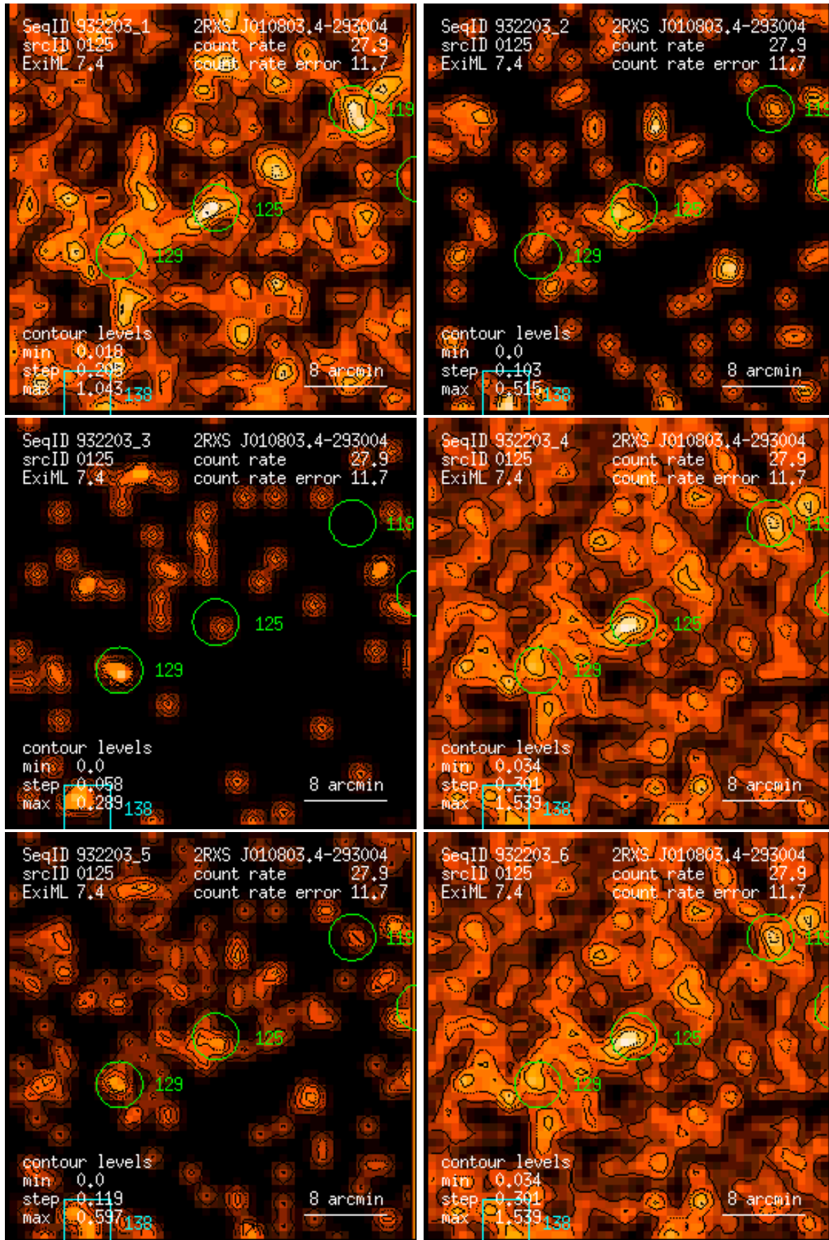
Figure 125: RASS 932203: detection 0125: band rate images, Gaussian filter: (1) PSPC channels 11 – 41, (2) 52 – 90, (3) 91 – 201, (4) 11 – 235, (5) 52 – 201, (6) 11 – 201. Broad band rates in counts/ks. Band rate contour levels in counts/ks/arcmin 2 .
