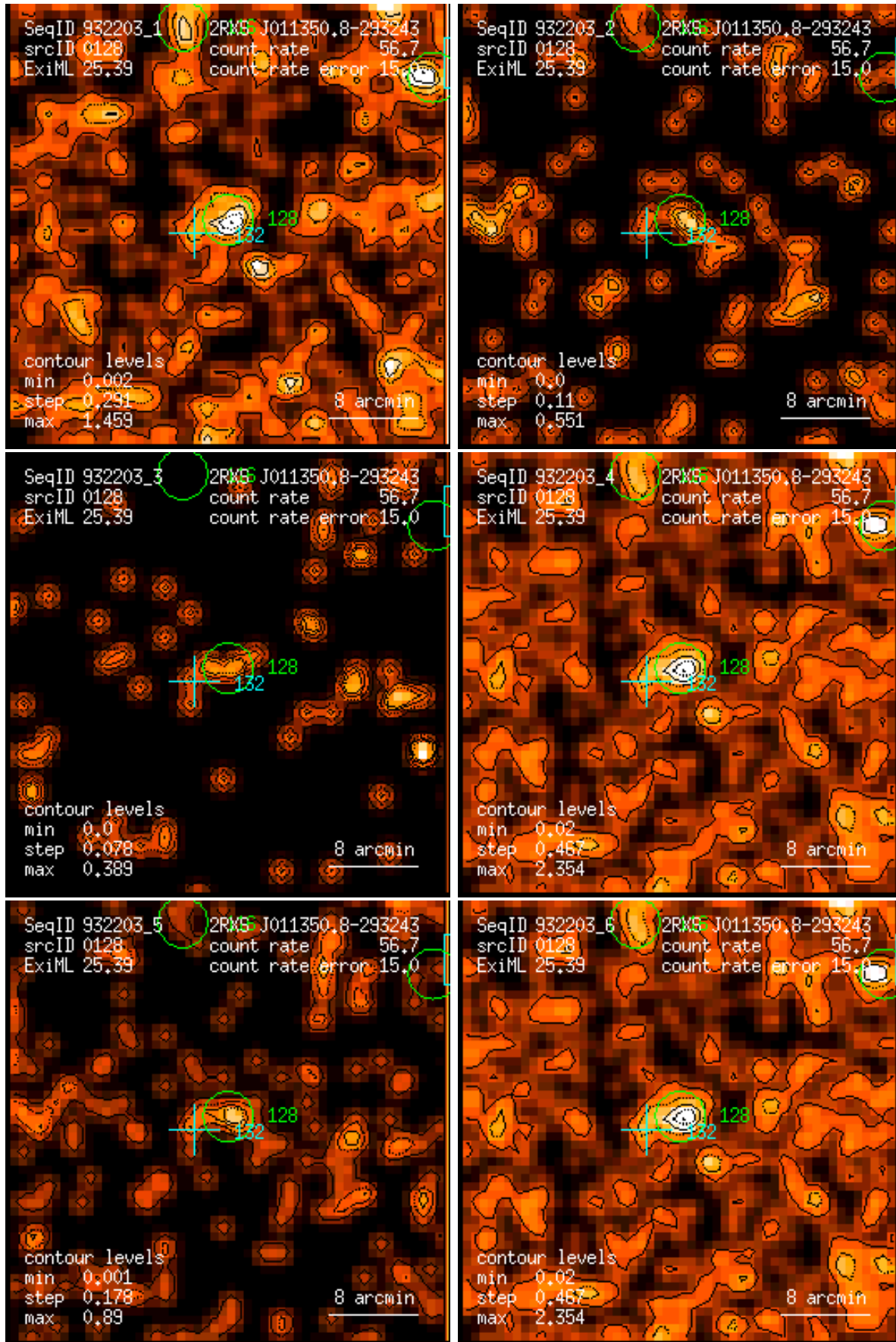
Figure 128: RASS 932203: detection 0128: band rate images, Gaussian filter: (1) PSPC channels 11 – 41, (2) 52 – 90, (3) 91 – 201, (4) 11 – 235, (5) 52 – 201, (6) 11 – 201. Broad band rates in counts/ks. Band rate contour levels in counts/ks/arcmin 2 .
