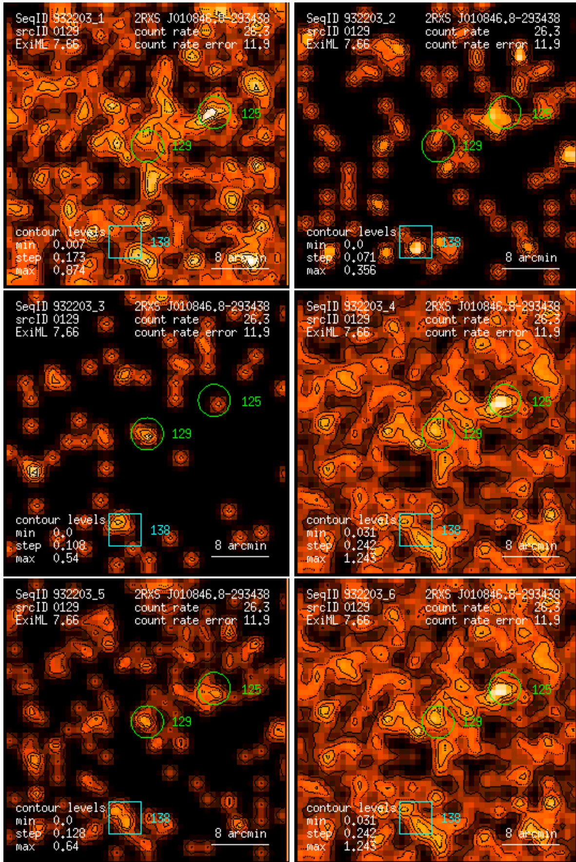
Figure 129: RASS 932203: detection 0129: band rate images, Gaussian filter: (1) PSPC channels 11 – 41, (2) 52 – 90, (3) 91 – 201, (4) 11 – 235, (5) 52 – 201, (6) 11 – 201. Broad band rates in counts/ks. Band rate contour levels in counts/ks/arcmin 2 .
