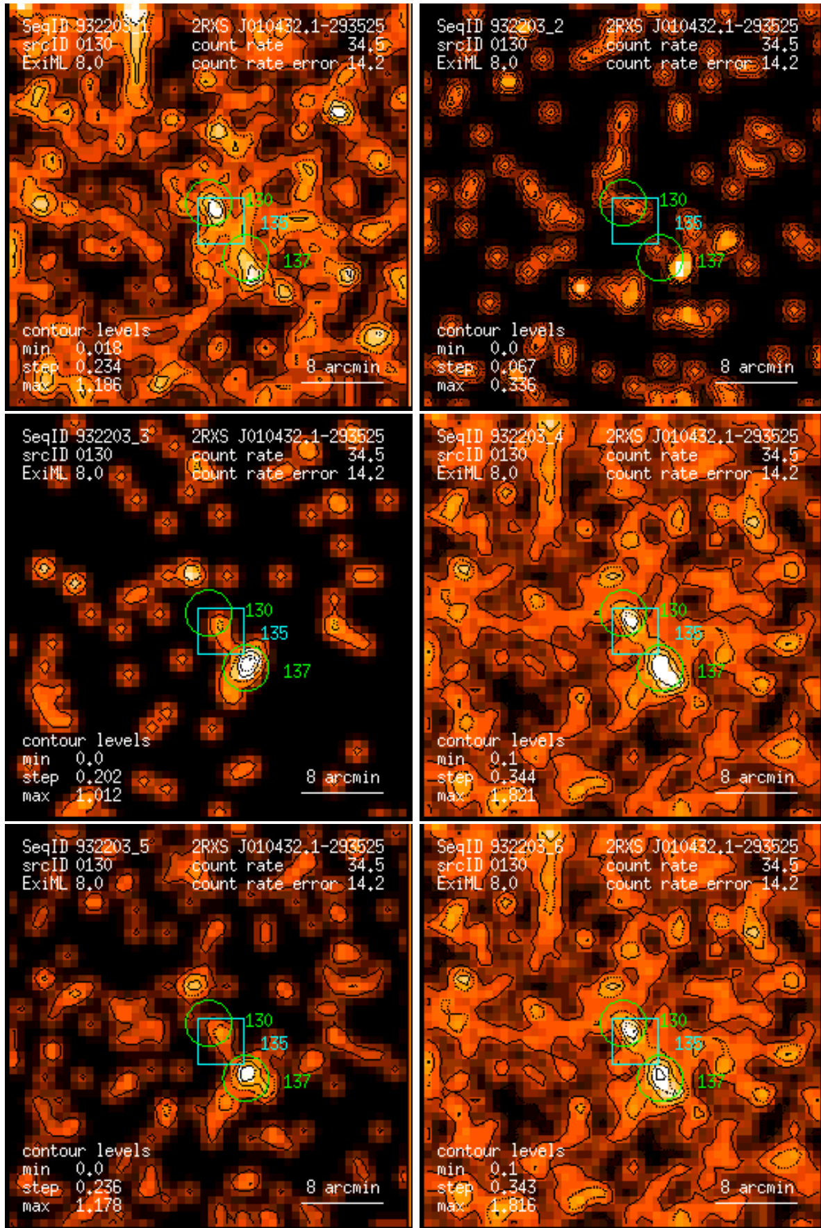
Figure 130: RASS 932203: detection 0130: band rate images, Gaussian filter: (1) PSPC channels 11 – 41, (2) 52 – 90, (3) 91 – 201, (4) 11 – 235, (5) 52 – 201, (6) 11 – 201. Broad band rates in counts/ks. Band rate contour levels in counts/ks/arcmin 2 .
