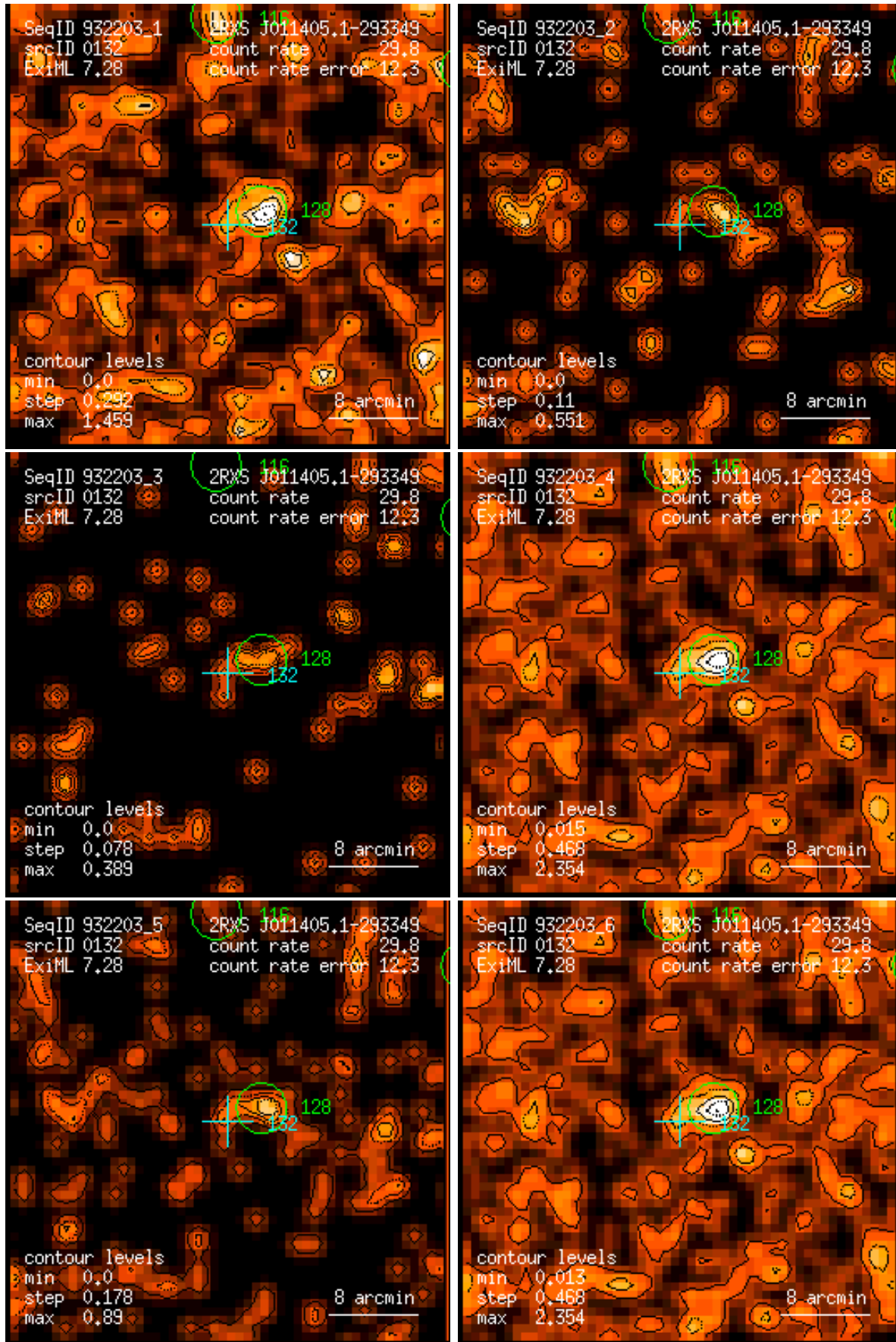
Figure 132: RASS 932203: detection 0132: band rate images, Gaussian filter: (1) PSPC channels 11 – 41, (2) 52 – 90, (3) 91 – 201, (4) 11 – 235, (5) 52 – 201, (6) 11 – 201. Broad band rates in counts/ks. Band rate contour levels in counts/ks/arcmin 2 .
