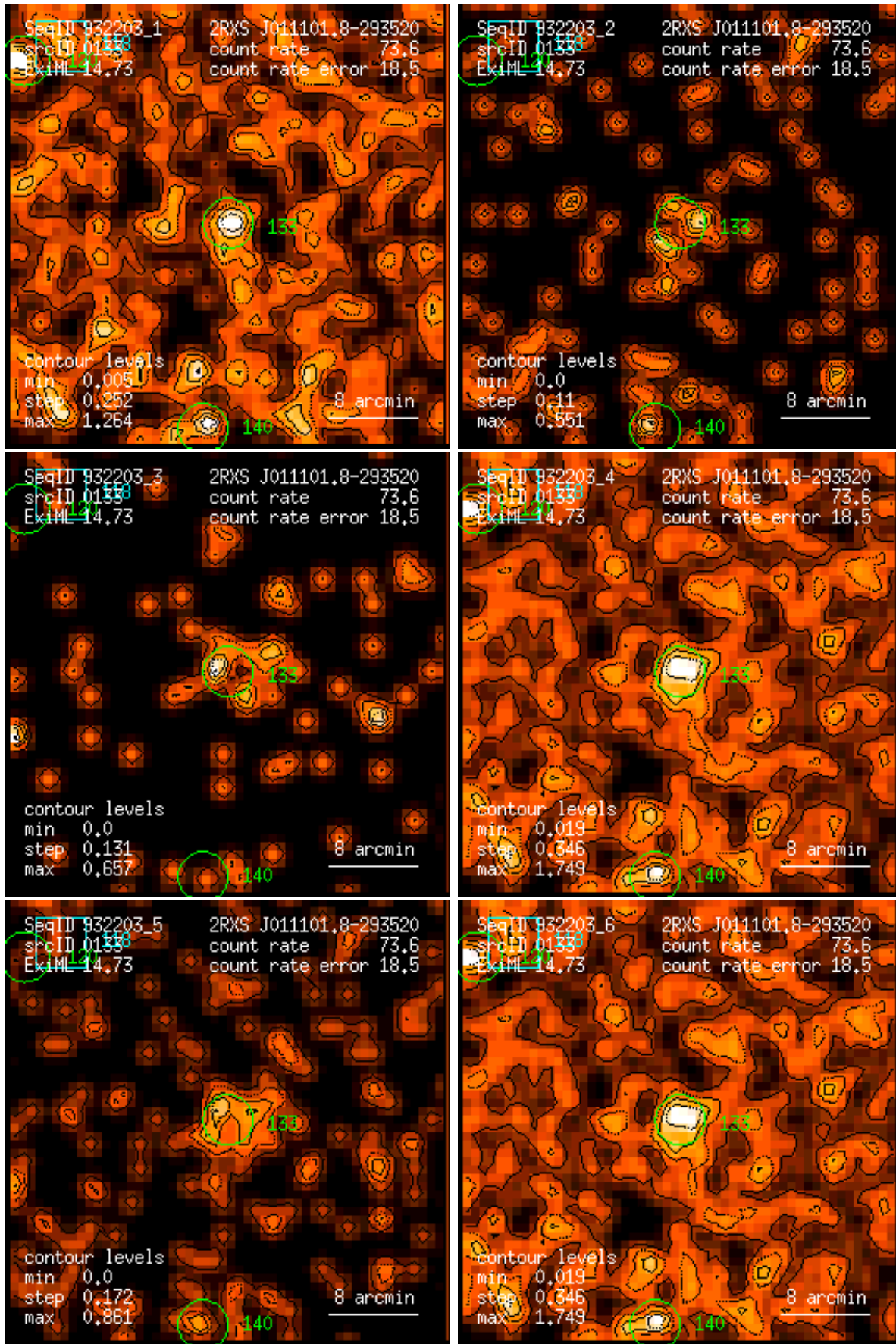
Figure 133: RASS 932203: detection 0133: band rate images, Gaussian filter: (1) PSPC channels 11 – 41, (2) 52 – 90, (3) 91 – 201, (4) 11 – 235, (5) 52 – 201, (6) 11 – 201. Broad band rates in counts/ks. Band rate contour levels in counts/ks/arcmin 2 .
