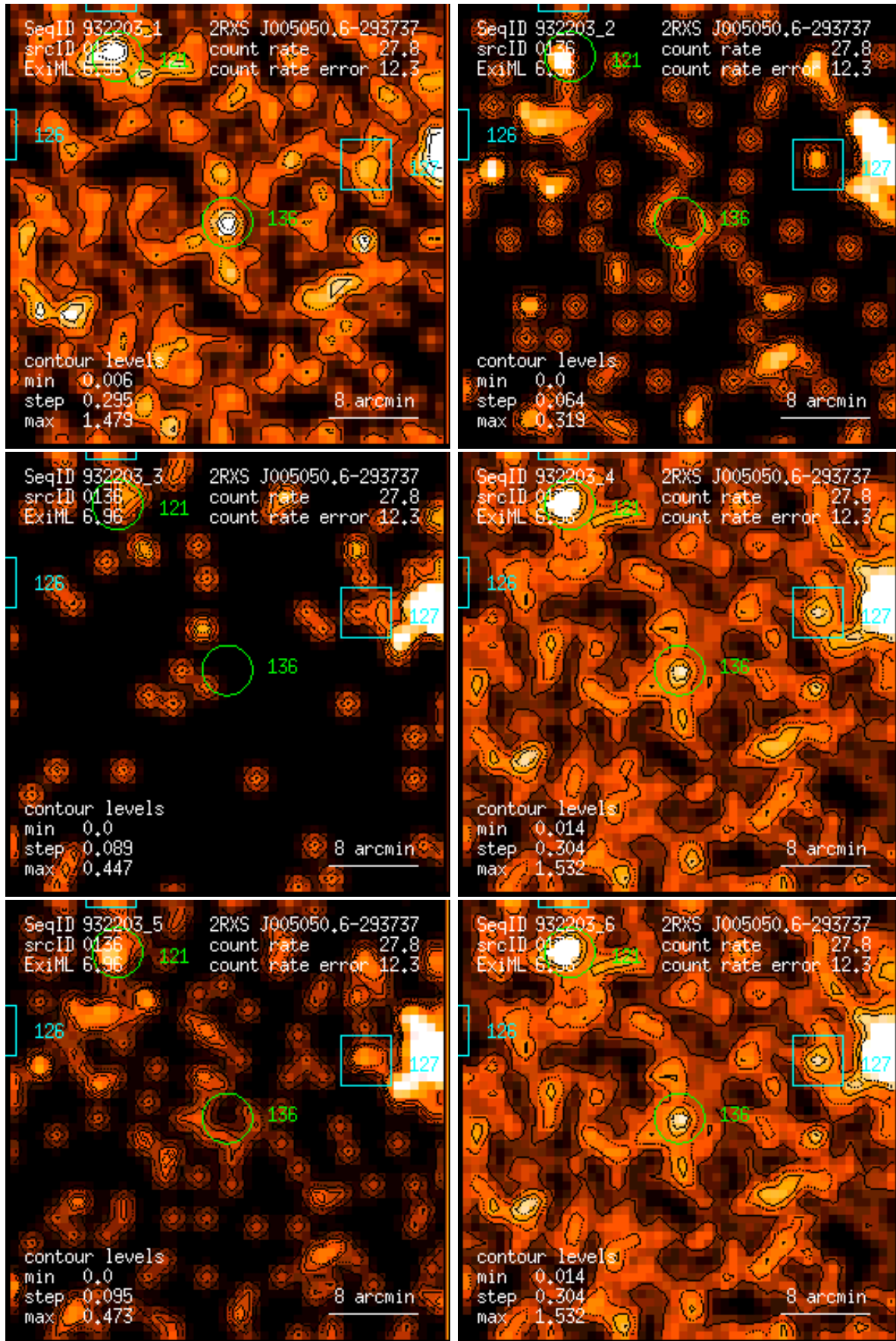
Figure 136: RASS 932203: detection 0136: band rate images, Gaussian filter: (1) PSPC channels 11 – 41, (2) 52 – 90, (3) 91 – 201, (4) 11 – 235, (5) 52 – 201, (6) 11 – 201. Broad band rates in counts/ks. Band rate contour levels in counts/ks/arcmin 2 .
