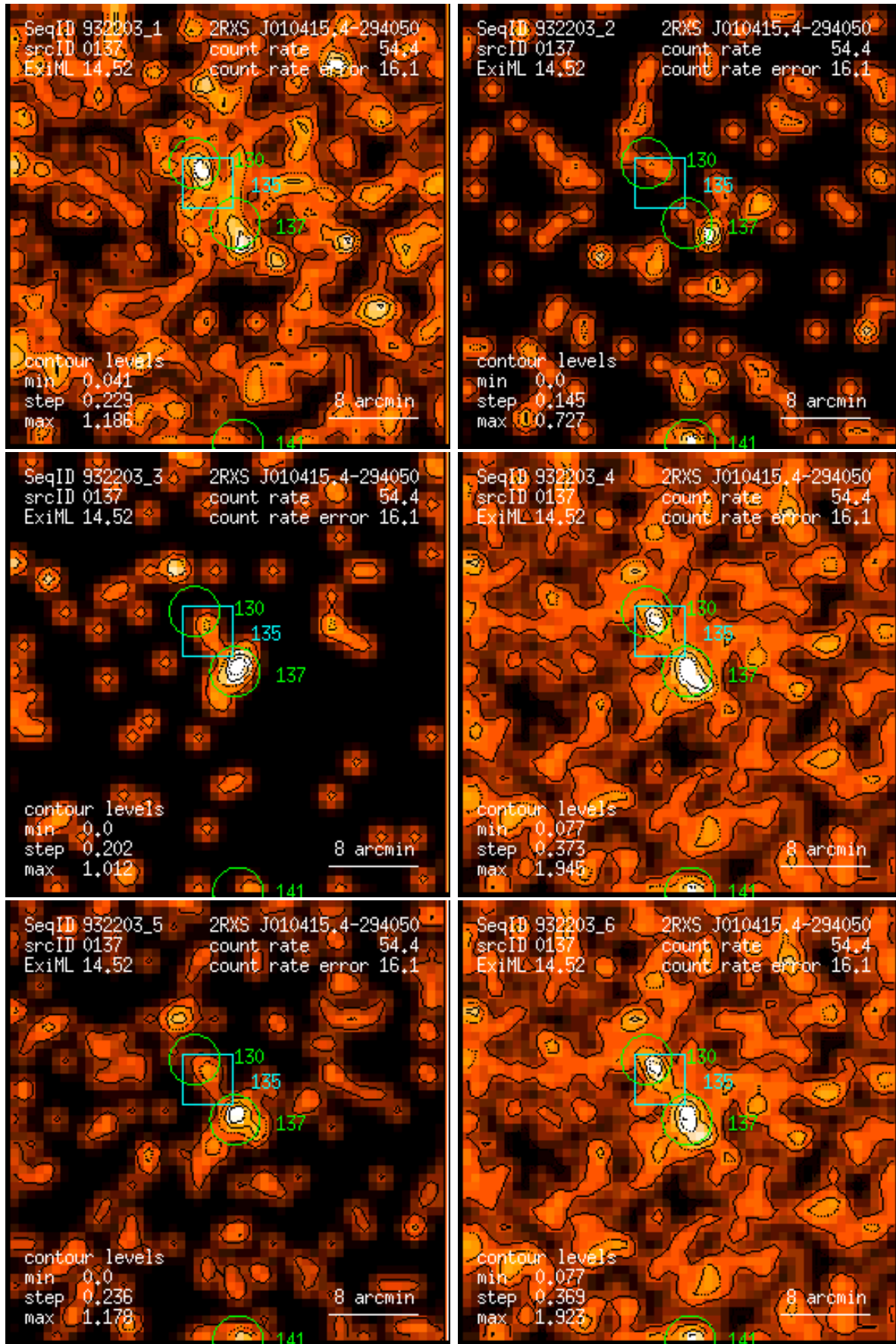
Figure 137: RASS 932203: detection 0137: band rate images, Gaussian filter: (1) PSPC channels 11 – 41, (2) 52 – 90, (3) 91 – 201, (4) 11 – 235, (5) 52 – 201, (6) 11 – 201. Broad band rates in counts/ks. Band rate contour levels in counts/ks/arcmin 2 .
