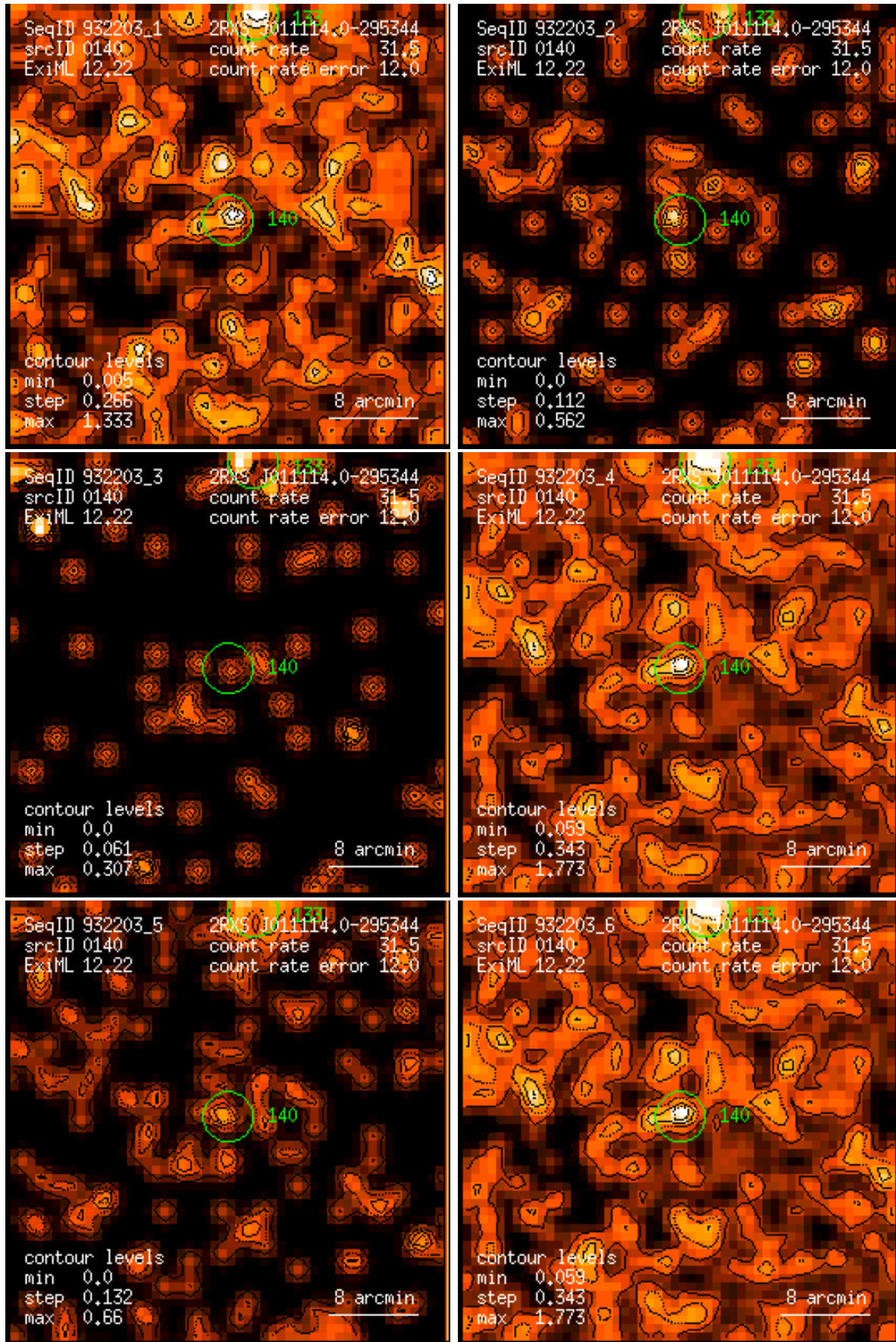
Figure 140: RASS 932203: detection 0140: band rate images, Gaussian filter: (1) PSPC channels 11 – 41, (2) 52 – 90, (3) 91 – 201, (4) 11 – 235, (5) 52 – 201, (6) 11 – 201. Broad band rates in counts/ks. Band rate contour levels in counts/ks/arcmin 2 .
