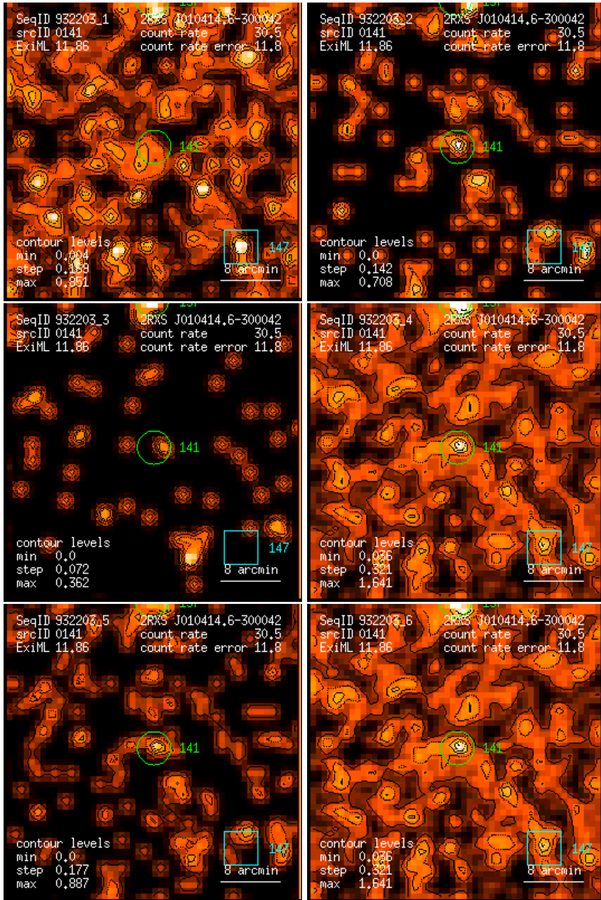
Figure 141: RASS 932203: detection 0141: band rate images, Gaussian filter: (1) PSPC channels 11 – 41, (2) 52 – 90, (3) 91 – 201, (4) 11 – 235, (5) 52 – 201, (6) 11 – 201. Broad band rates in counts/ks. Band rate contour levels in counts/ks/arcmin 2 .
