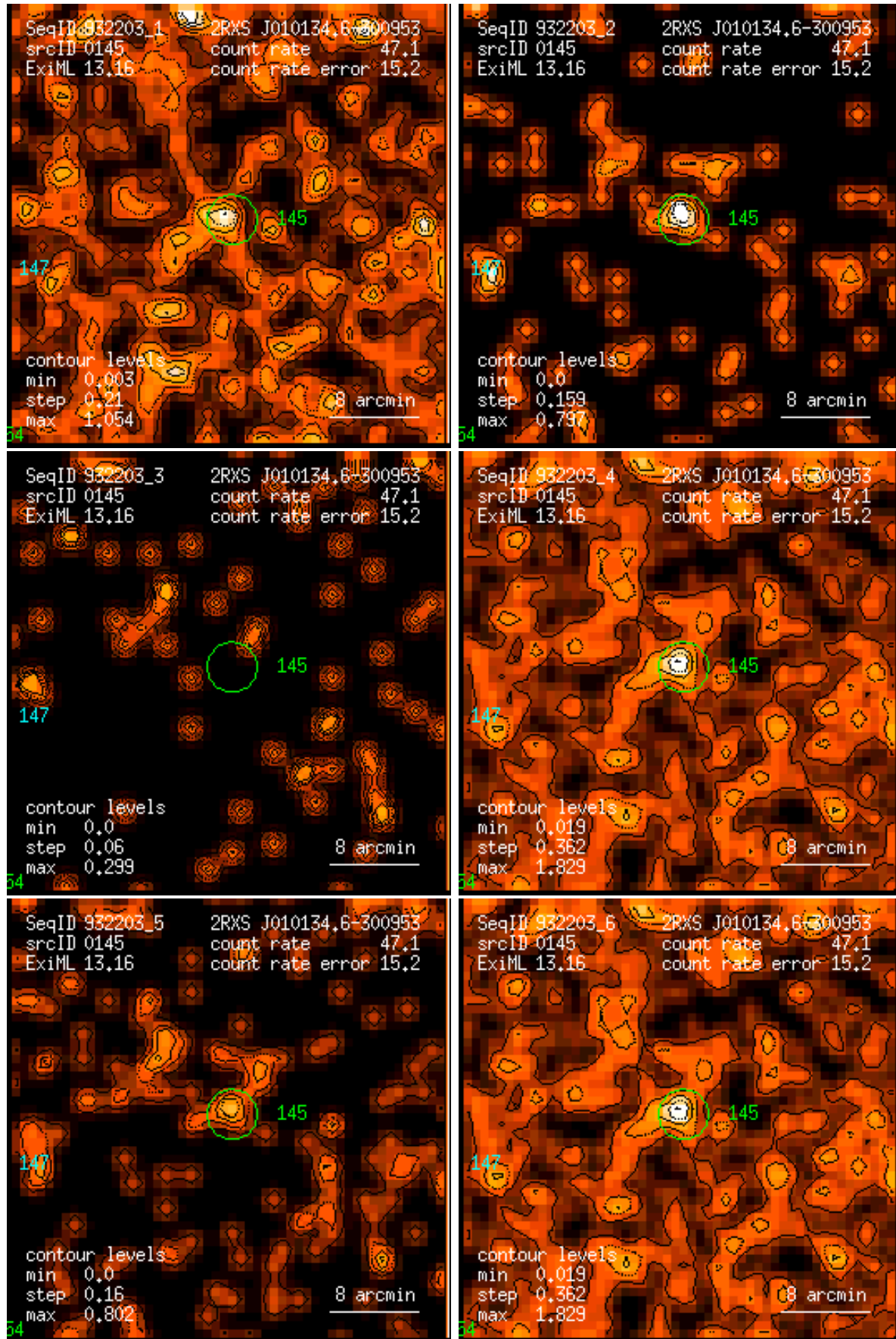
Figure 145: RASS 932203: detection 0145: band rate images, Gaussian filter: (1) PSPC channels 11 – 41, (2) 52 – 90, (3) 91 – 201, (4) 11 – 235, (5) 52 – 201, (6) 11 – 201. Broad band rates in counts/ks. Band rate contour levels in counts/ks/arcmin 2 .
