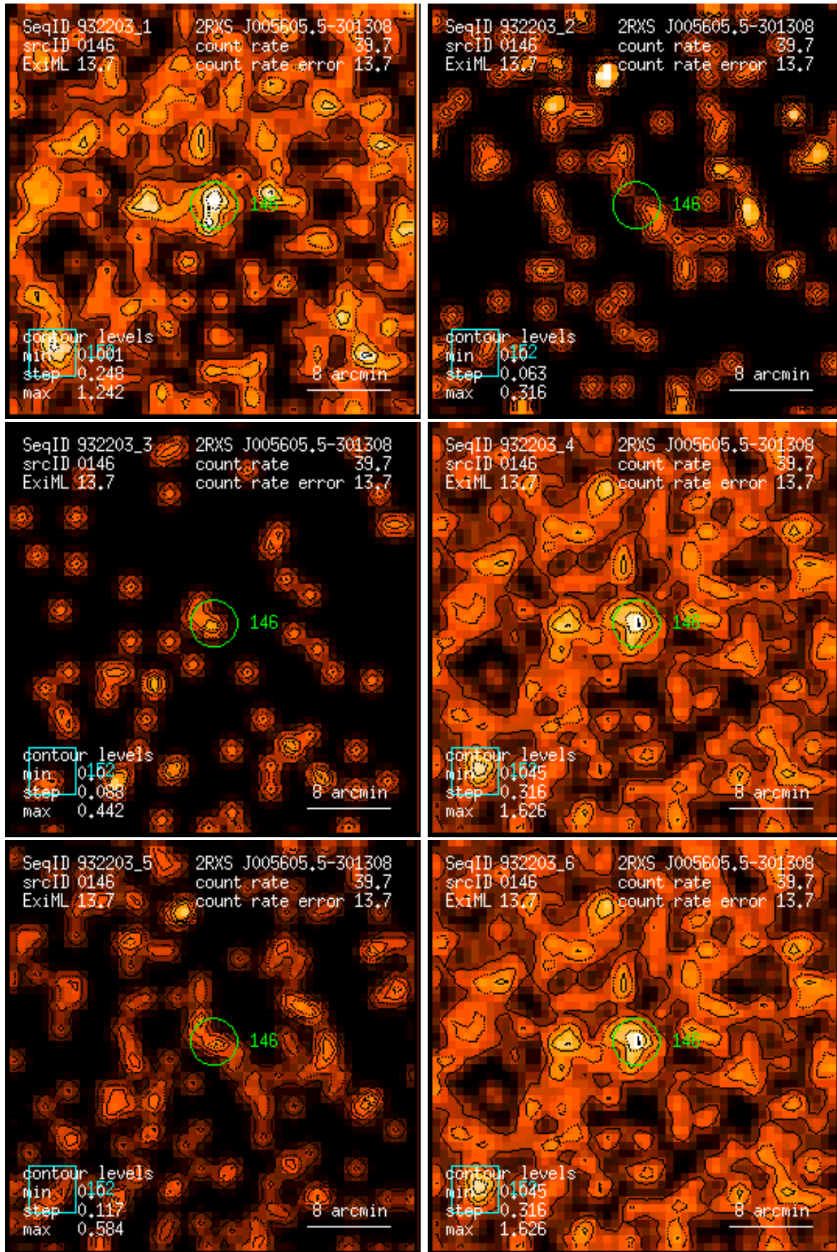
Figure 146: RASS 932203: detection 0146: band rate images, Gaussian filter: (1) PSPC channels 11 – 41, (2) 52 – 90, (3) 91 – 201, (4) 11 – 235, (5) 52 – 201, (6) 11 – 201. Broad band rates in counts/ks. Band rate contour levels in counts/ks/arcmin 2 .
