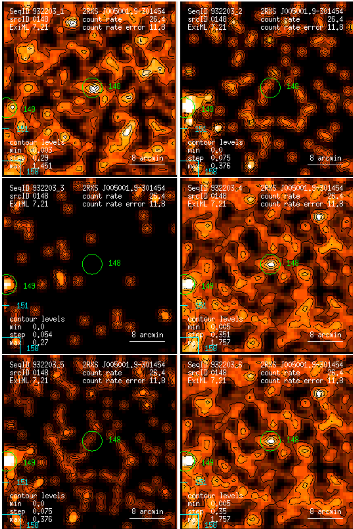
Figure 148: RASS 932203: detection 0148: band rate images, Gaussian filter: (1) PSPC channels 11 – 41, (2) 52 – 90, (3) 91 – 201, (4) 11 – 235, (5) 52 – 201, (6) 11 – 201. Broad band rates in counts/ks. Band rate contour levels in counts/ks/arcmin 2 .
