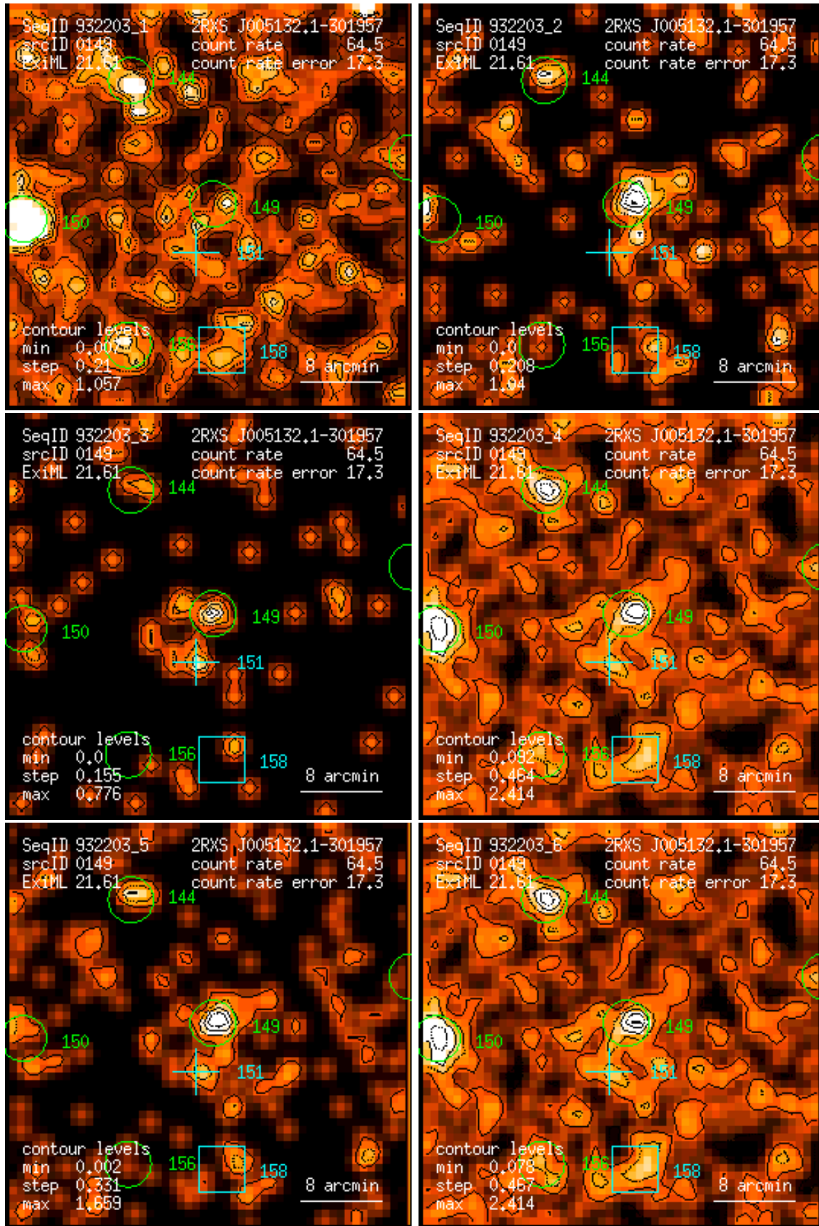
Figure 149: RASS 932203: detection 0149: band rate images, Gaussian filter: (1) PSPC channels 11 – 41, (2) 52 – 90, (3) 91 – 201, (4) 11 – 235, (5) 52 – 201, (6) 11 – 201. Broad band rates in counts/ks. Band rate contour levels in counts/ks/arcmin 2 .
