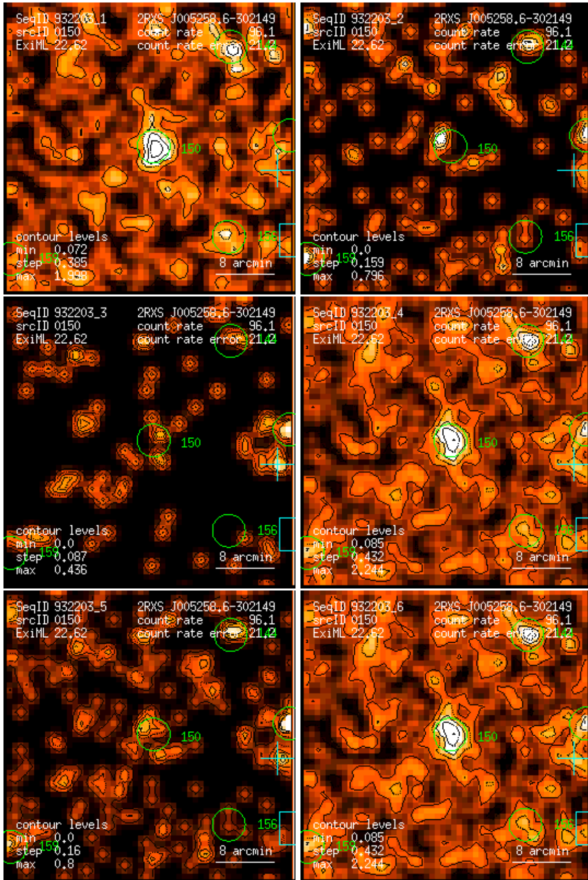
Figure 150: RASS 932203: detection 0150: band rate images, Gaussian filter: (1) PSPC channels 11 – 41, (2) 52 – 90, (3) 91 – 201, (4) 11 – 235, (5) 52 – 201, (6) 11 – 201. Broad band rates in counts/ks. Band rate contour levels in counts/ks/arcmin 2 .
