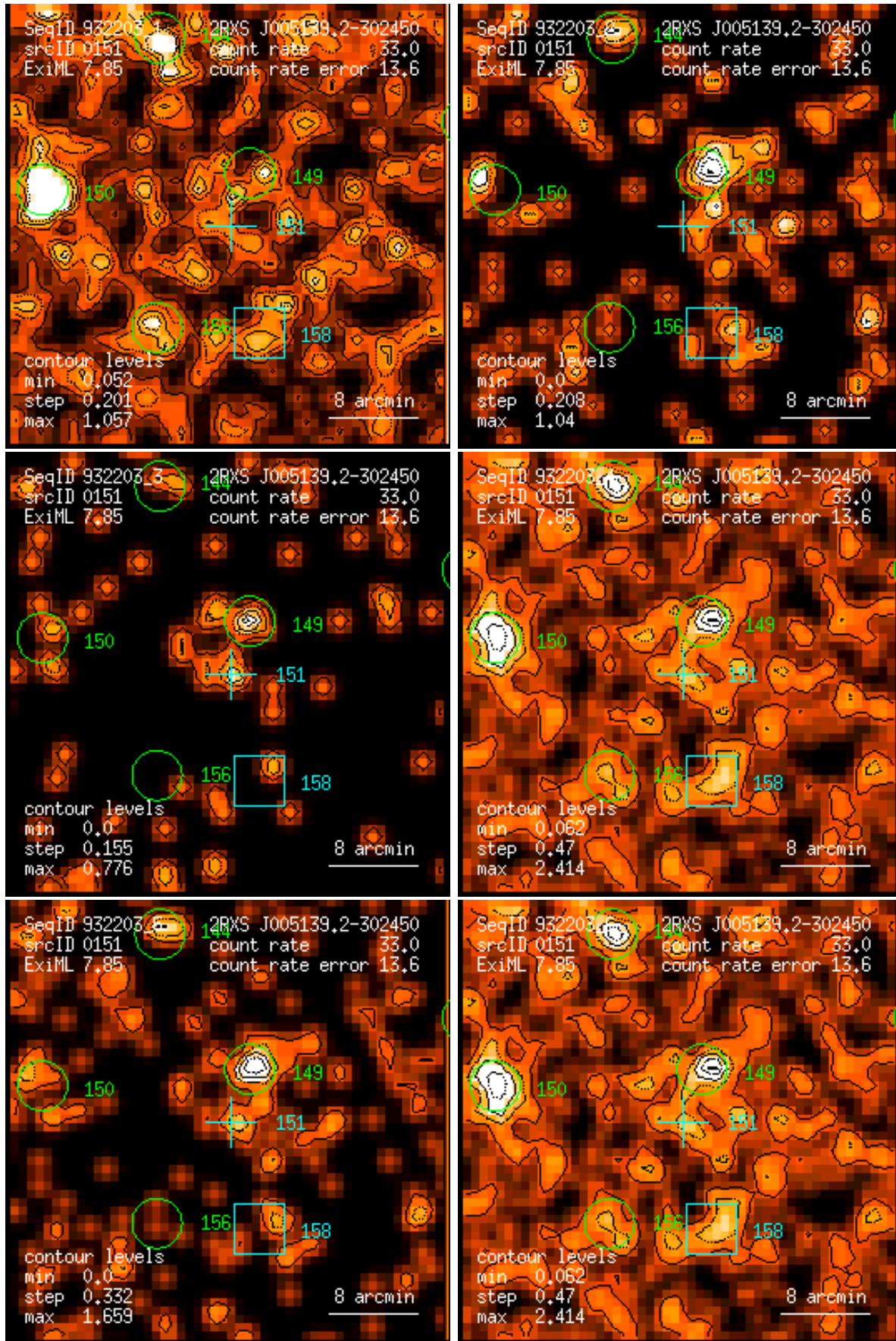
Figure 151: RASS 932203: detection 0151: band rate images, Gaussian filter: (1) PSPC channels 11 – 41, (2) 52 – 90, (3) 91 – 201, (4) 11 – 235, (5) 52 – 201, (6) 11 – 201. Broad band rates in counts/ks. Band rate contour levels in counts/ks/arcmin 2 .
