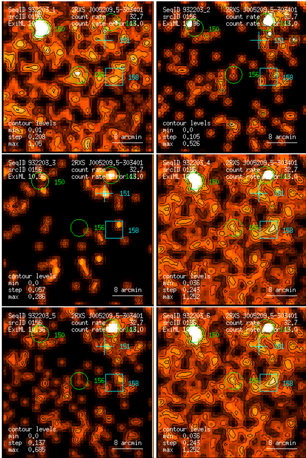
Figure 156: RASS 932203: detection 0156: band rate images, Gaussian filter: (1) PSPC channels 11 – 41, (2) 52 – 90, (3) 91 – 201, (4) 11 – 235, (5) 52 – 201, (6) 11 – 201. Broad band rates in counts/ks. Band rate contour levels in counts/ks/arcmin 2 .
