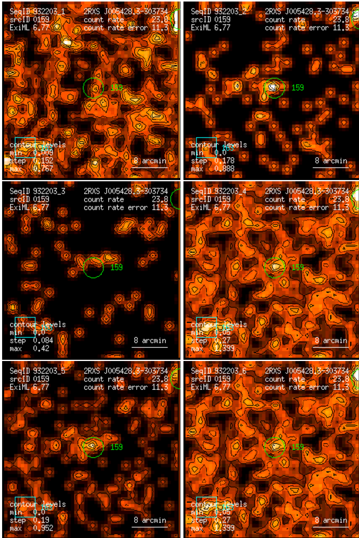
Figure 159: RASS 932203: detection 0159: band rate images, Gaussian filter: (1) PSPC channels 11 – 41, (2) 52 – 90, (3) 91 – 201, (4) 11 – 235, (5) 52 – 201, (6) 11 – 201. Broad band rates in counts/ks. Band rate contour levels in counts/ks/arcmin 2 .
