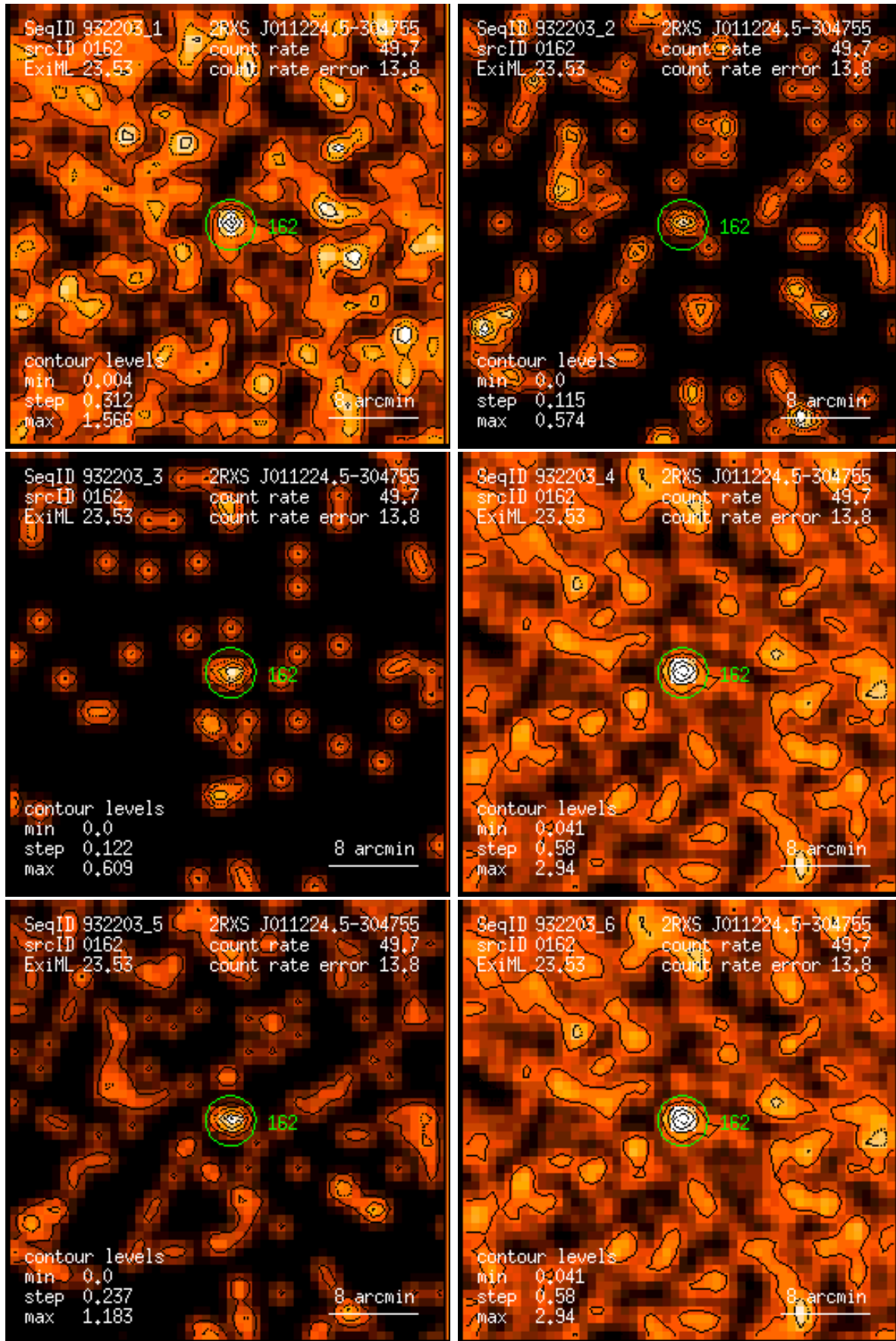
Figure 162: RASS 932203: detection 0162: band rate images, Gaussian filter: (1) PSPC channels 11 – 41, (2) 52 – 90, (3) 91 – 201, (4) 11 – 235, (5) 52 – 201, (6) 11 – 201. Broad band rates in counts/ks. Band rate contour levels in counts/ks/arcmin 2 .
