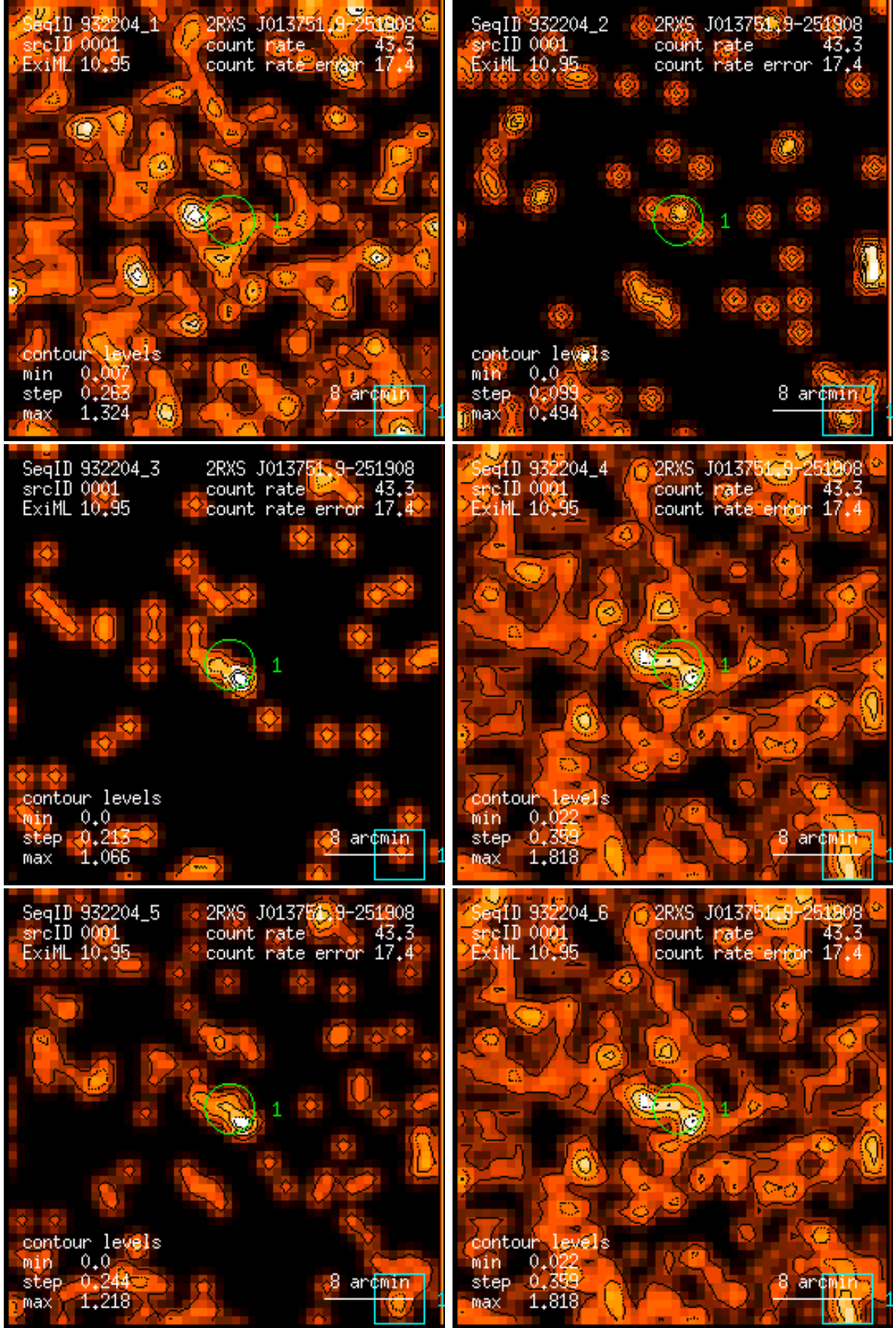
Figure 1: RASS 932204: detection 0001: band rate images, Gaussian filter: (1) PSPC channels 11 – 41, (2) 52 – 90, (3) 91 – 201, (4) 11 – 235, (5) 52 – 201, (6) 11 – 201. Broad band rates in counts/ks. Band rate contour levels in counts/ks/arcmin 2 .
